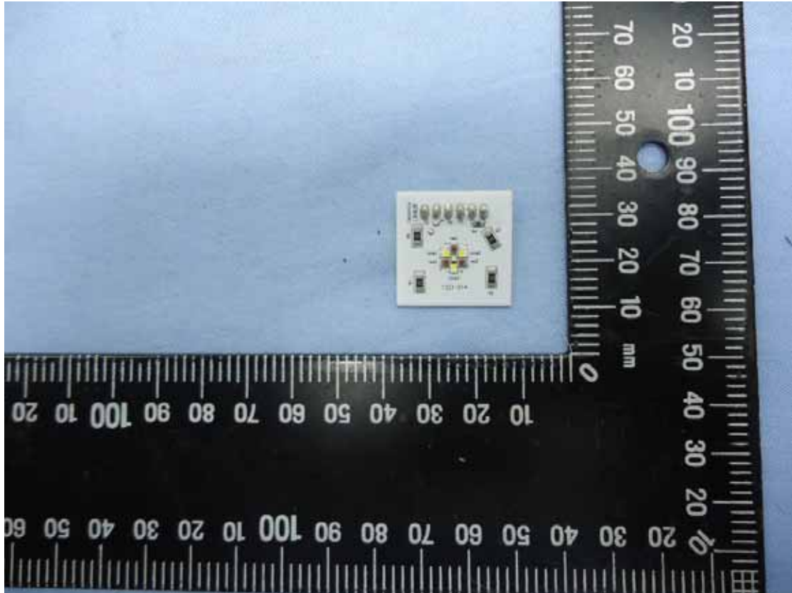
Figure 9 LED Board
