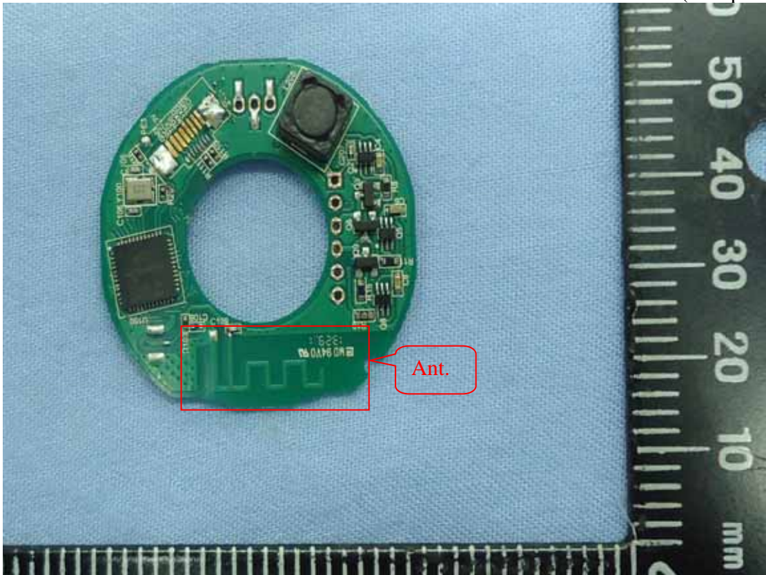
Figure 6 Wireless Board (Component Side)
