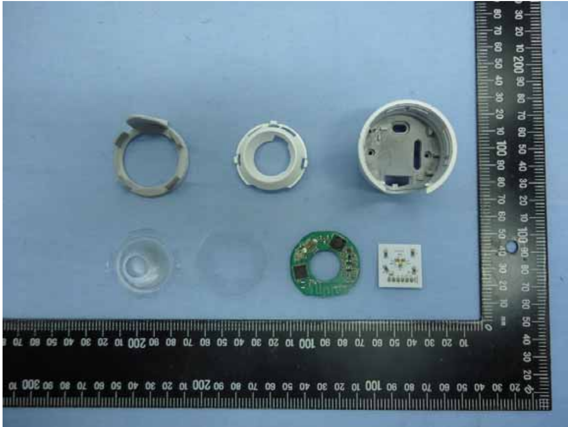
Figure 5 Internal View
