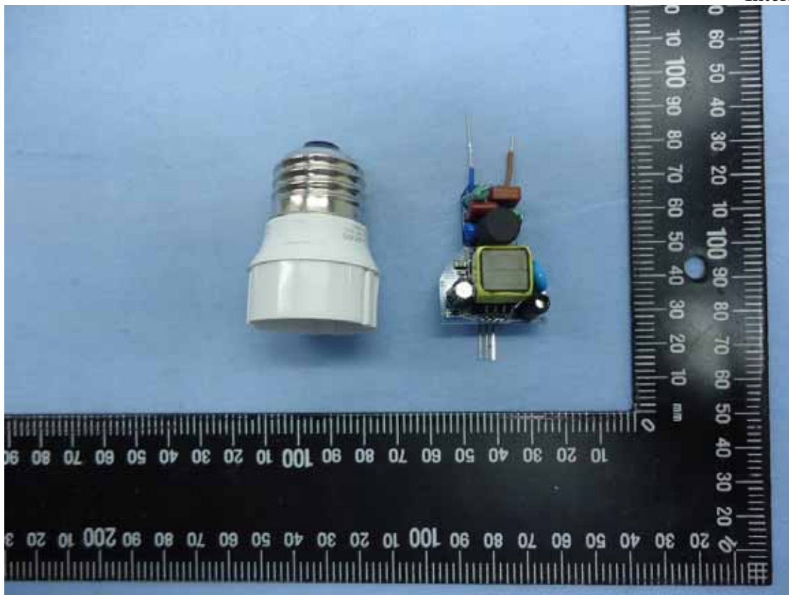
Figure 2 Internal View
