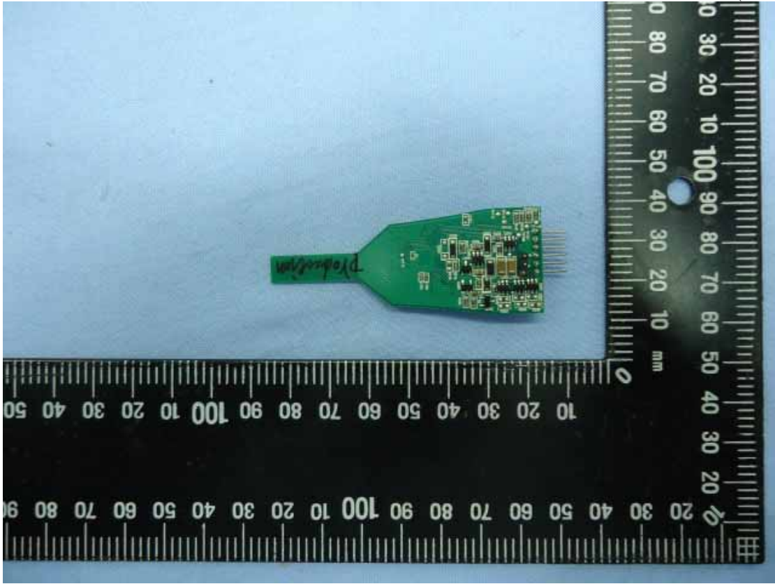
Figure 6 LED Board (Component Side)
