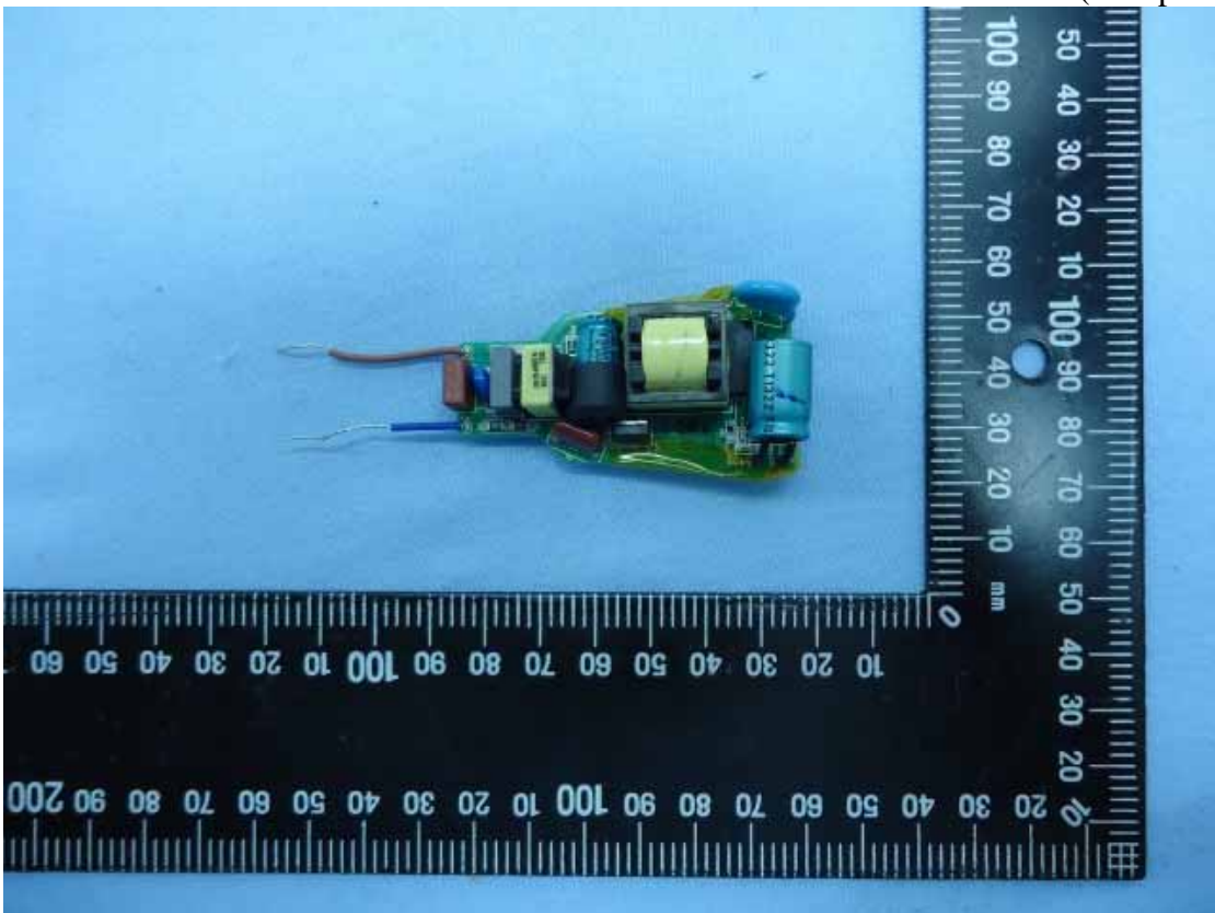
Figure 2 Power Board (Component Side)
