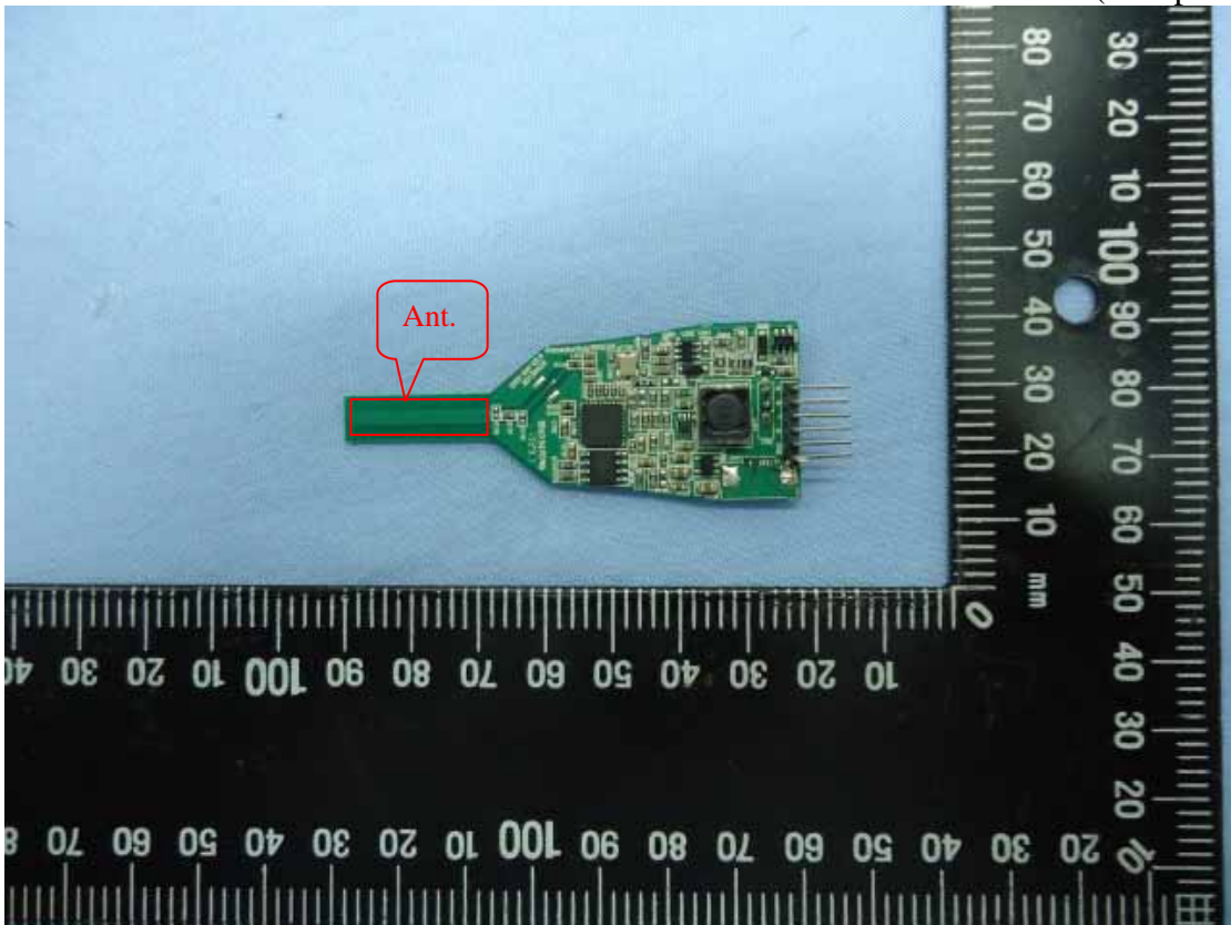
Figure 4 Wireless Board (Component Side)
