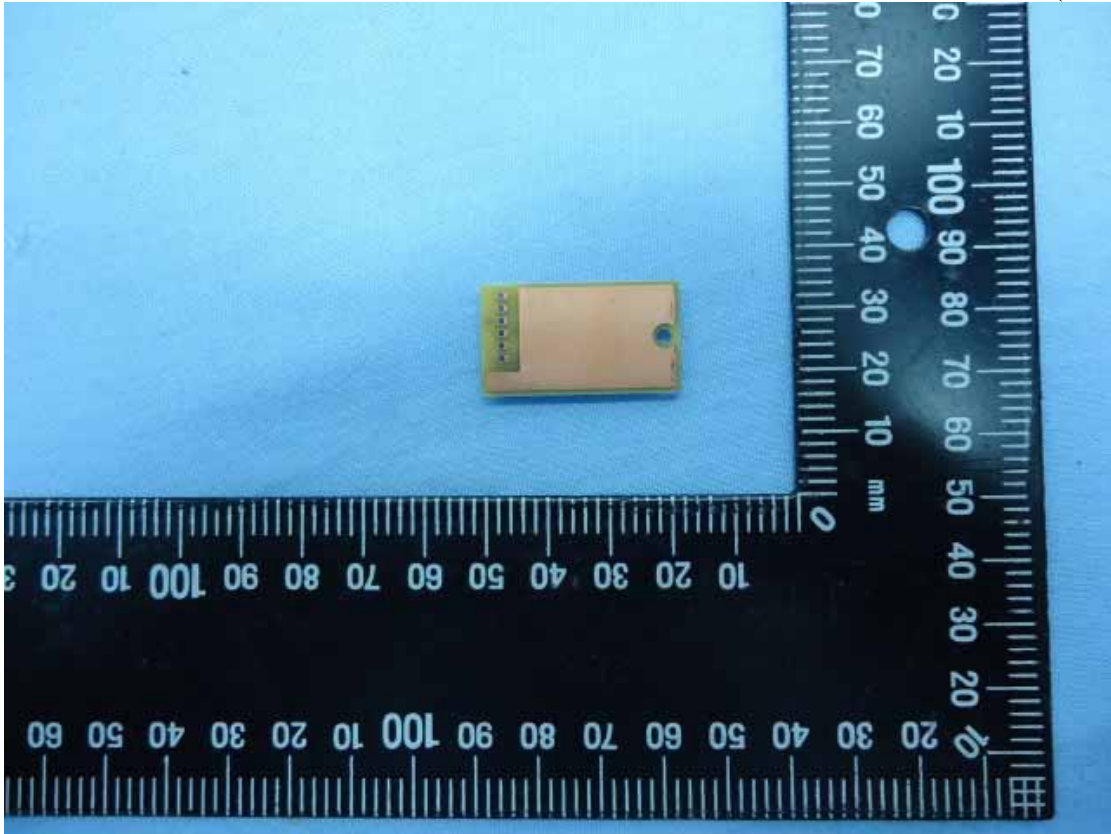
Figure 7 LED Board (Solder Side)
