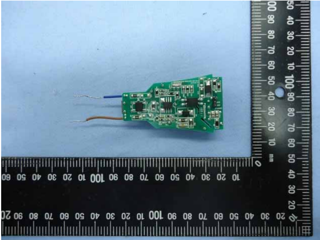
Figure 3 Power Board (Solder Side)
