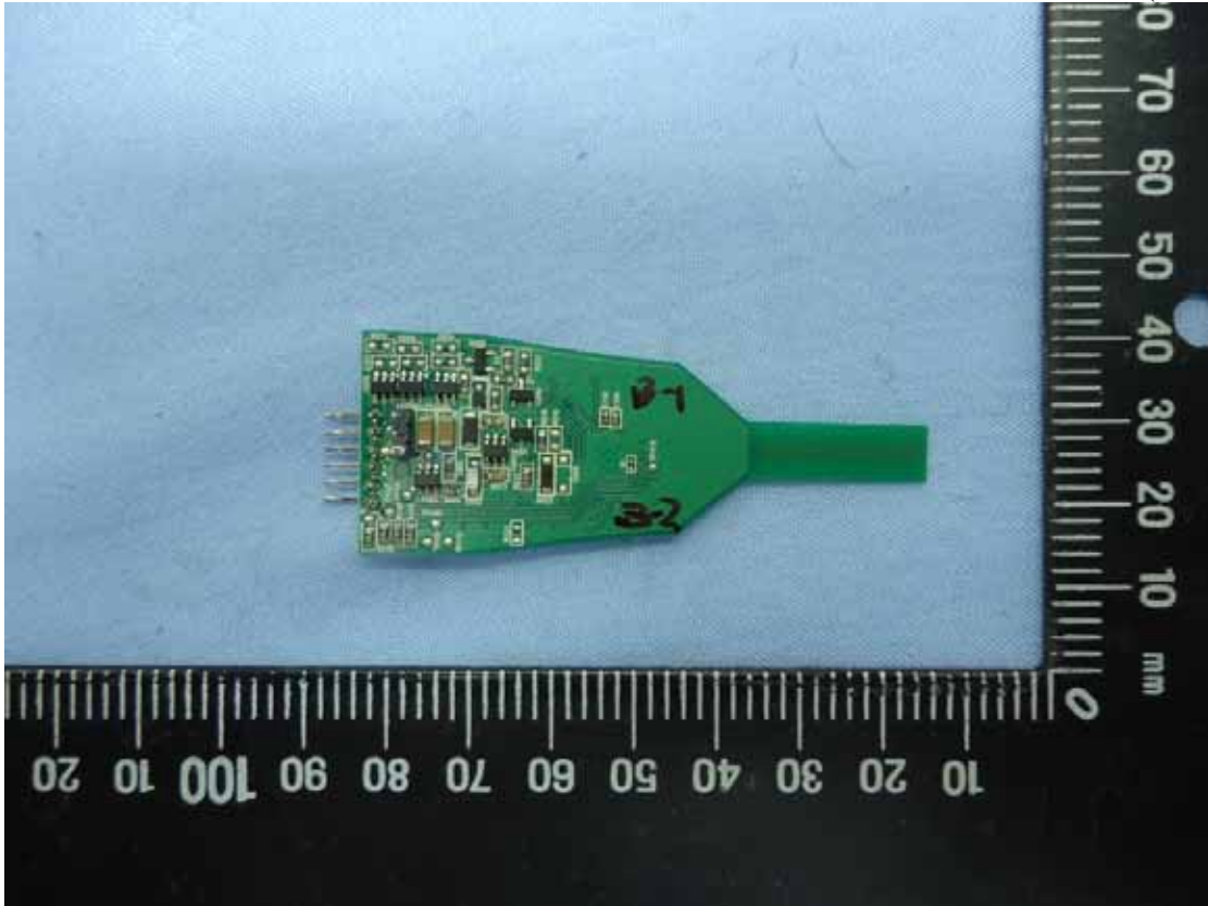
Figure 5 Wireless Board (Solder Side)
