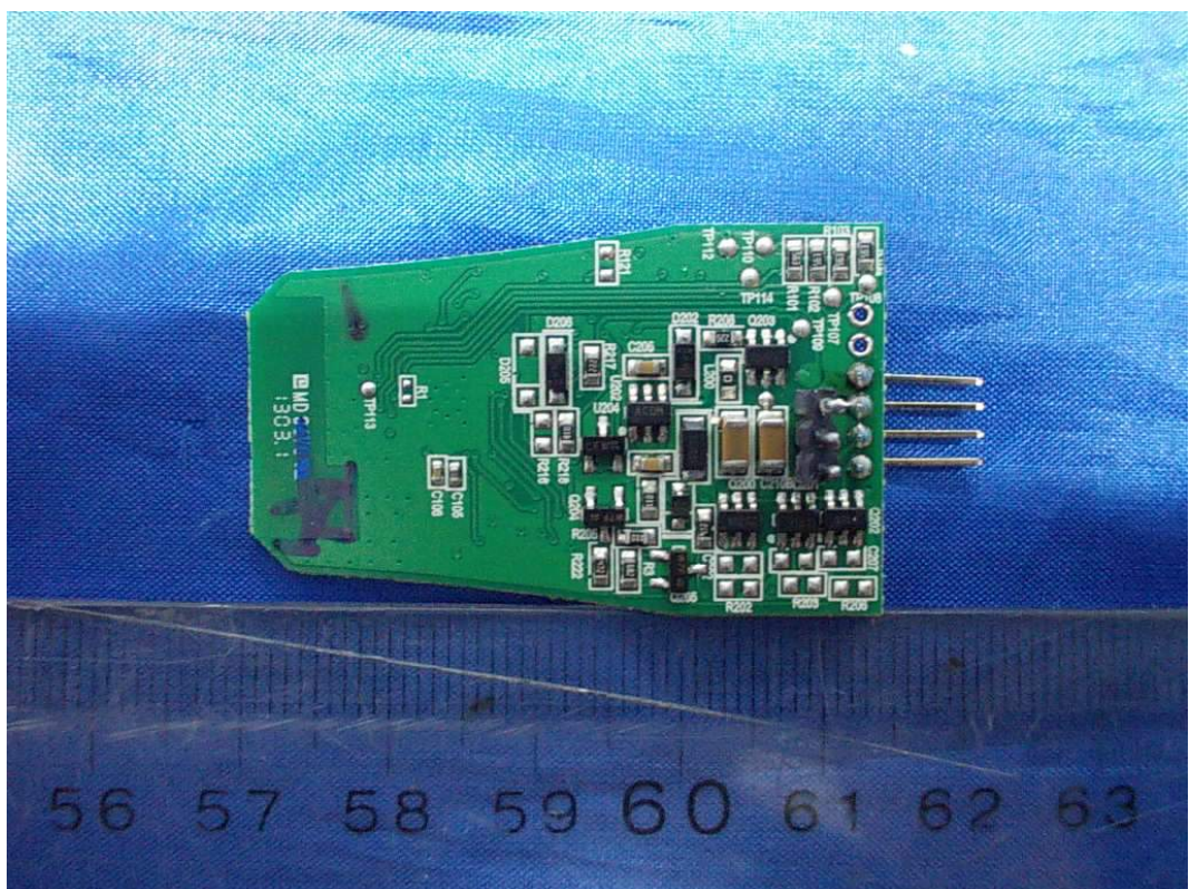
FIGURE 8 LED LAMPS (M/N: 9290002265) RF BOARD (BACK VIEW)
