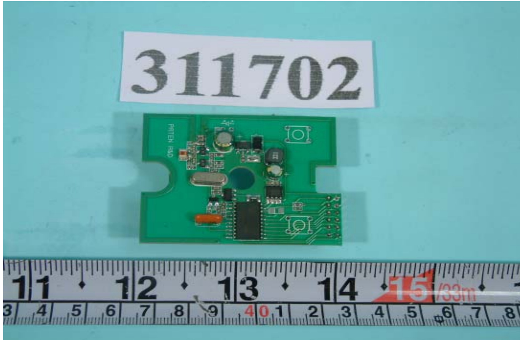
Front side of Main Board
