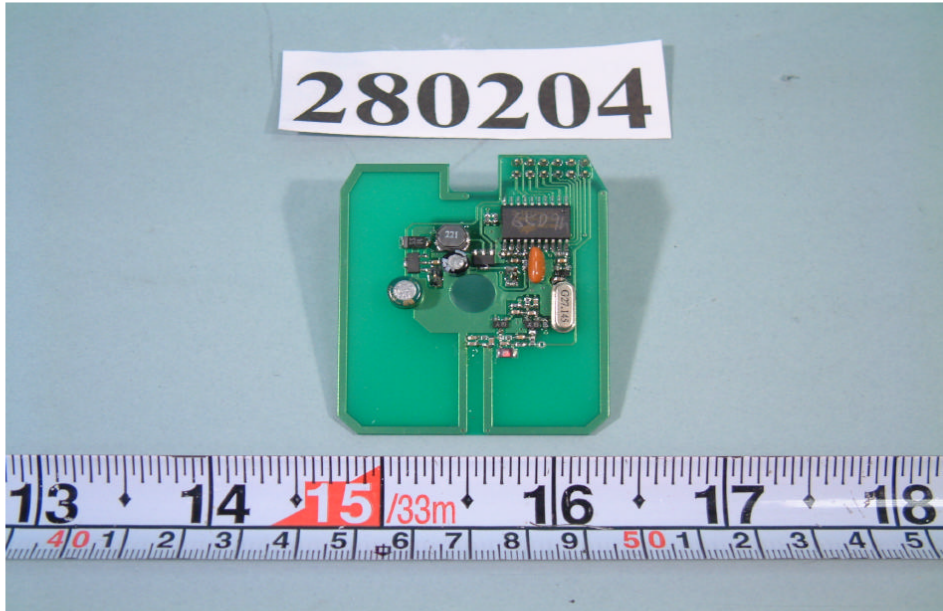
Front side of Main Board Of Mouse
