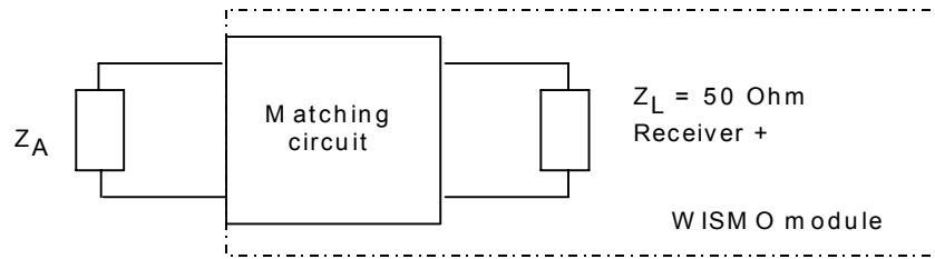
Figure 7: Matching circuit
