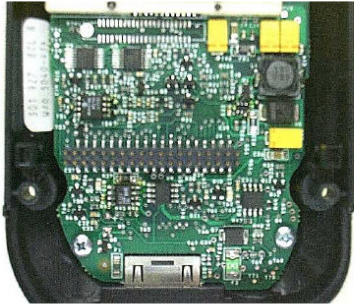
Bottom third of Transmitter board
