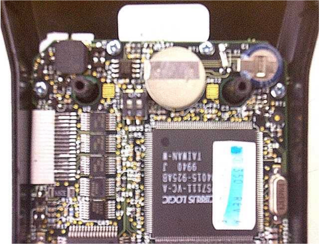
Top of rear of keyboard
