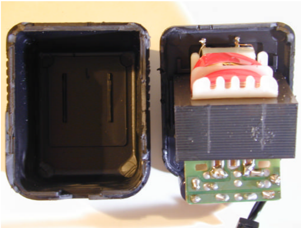
(22) EUT Photo
