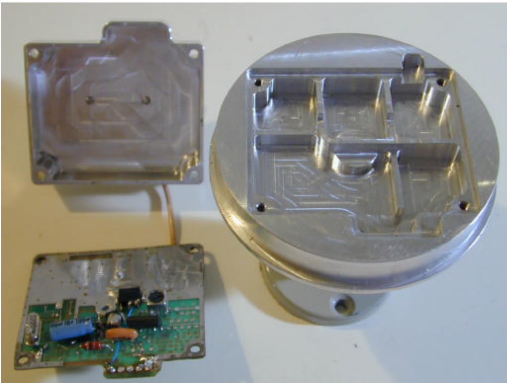
(26) EUT Photo
