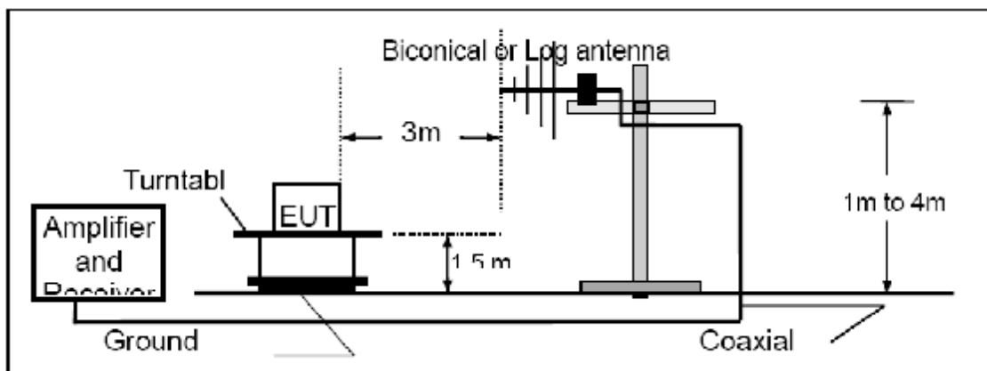
TEST SETUP BELOW 1GHZ
