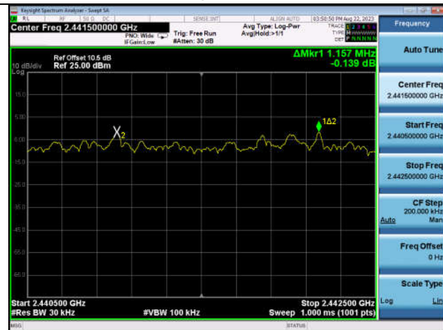
DQPSK,Hopping2DH5,2440.5~2442.5
