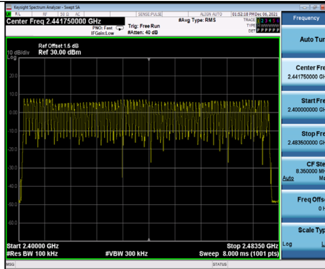
GFSK Modulation
