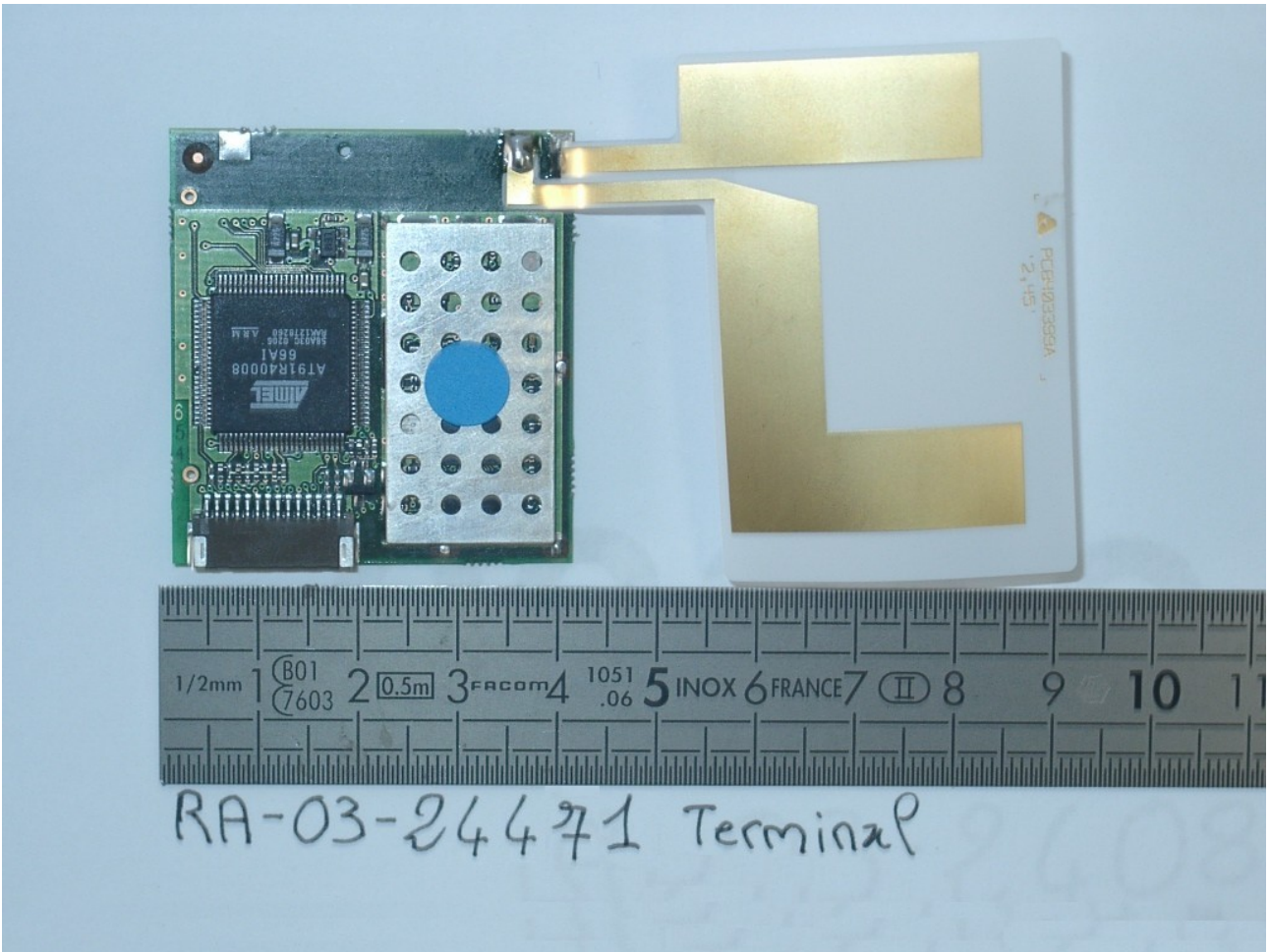
Printed circuit board transmitter: face 3
