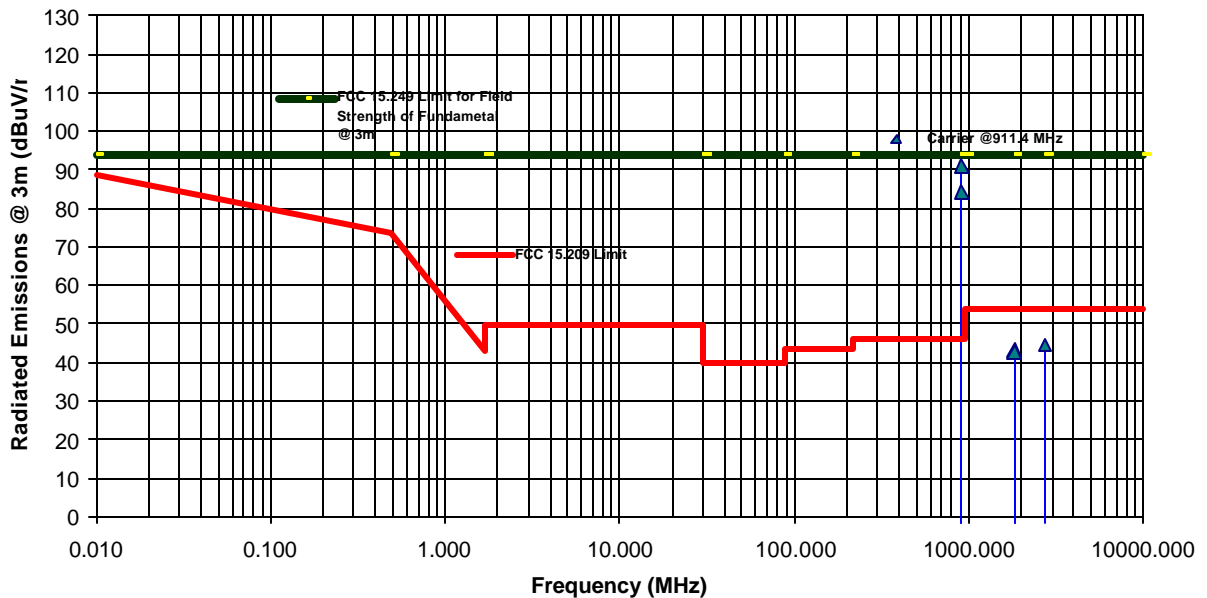
Transmitter Radiated Emissions Measurements at 3 Meters OFTS TRANSMIT Freq.: 911.4 MHz IVI Checkmate Inc. Elite 770 Intelligent Base, Model Elite 770 Intelligent Base
