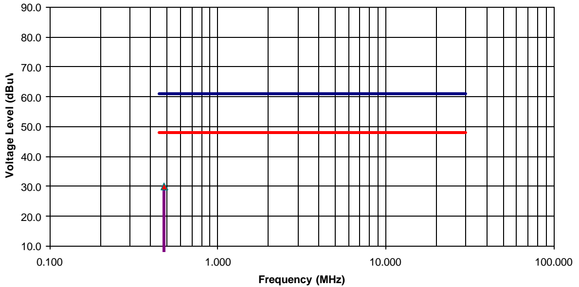
AC Conducted Emissions - Line #1 (Hot) IVI Checkmate Inc. Elite 770 Intelligent Base, Model Elite 770 Intelligent Base
