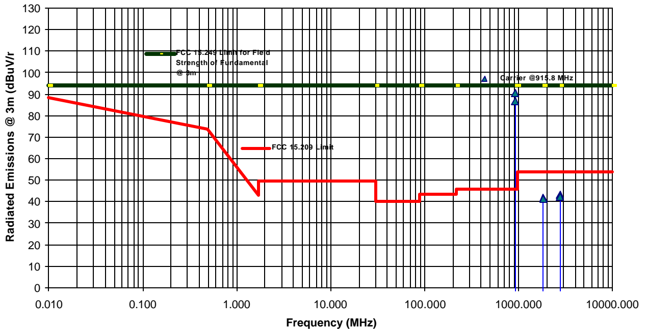
Transmitter Radiated Emissions Measurements at 3 Meters OETS TRANSMIT Freq.: 915.8MHz IVI Checkmate Inc. Elite 770 Intelligent Base, Model Elite 770 Intelligent Base
