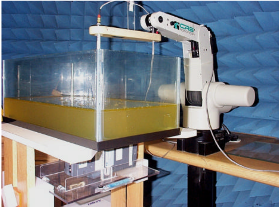
Figure 1. Setup
