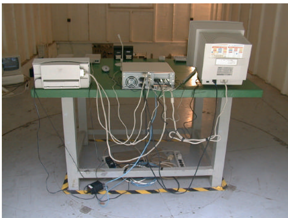
Back View of Radiated Emission Test (Mode 1)
