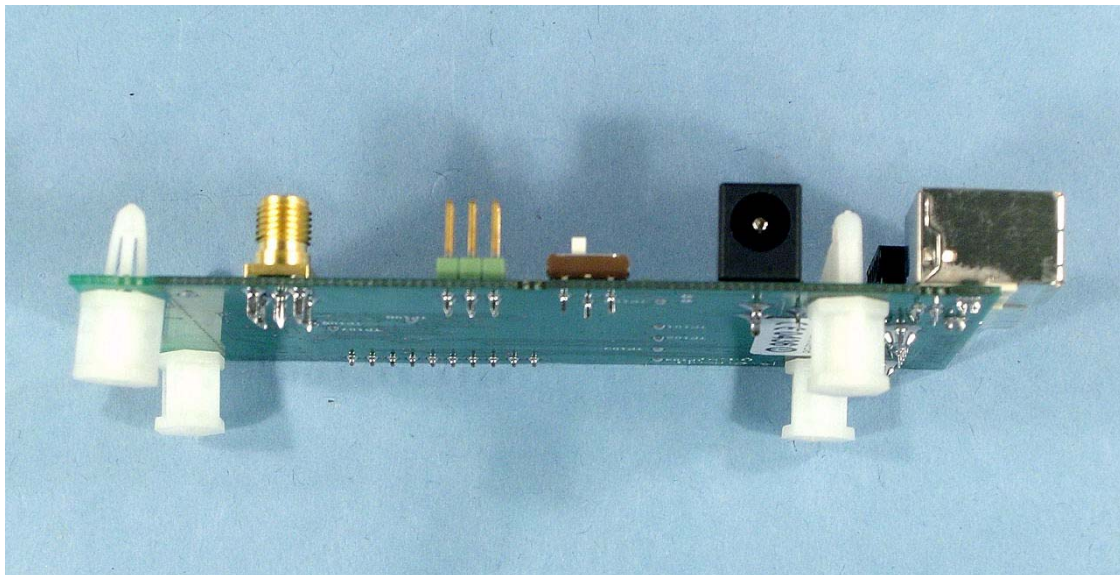
13192-EVB, view of power connector
