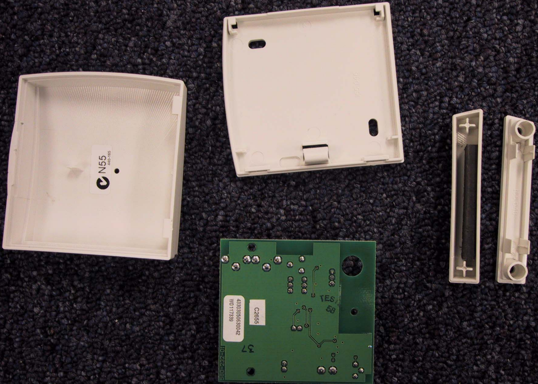
106-065 RR2 Wireless Universal Transmitter Inside Back View
