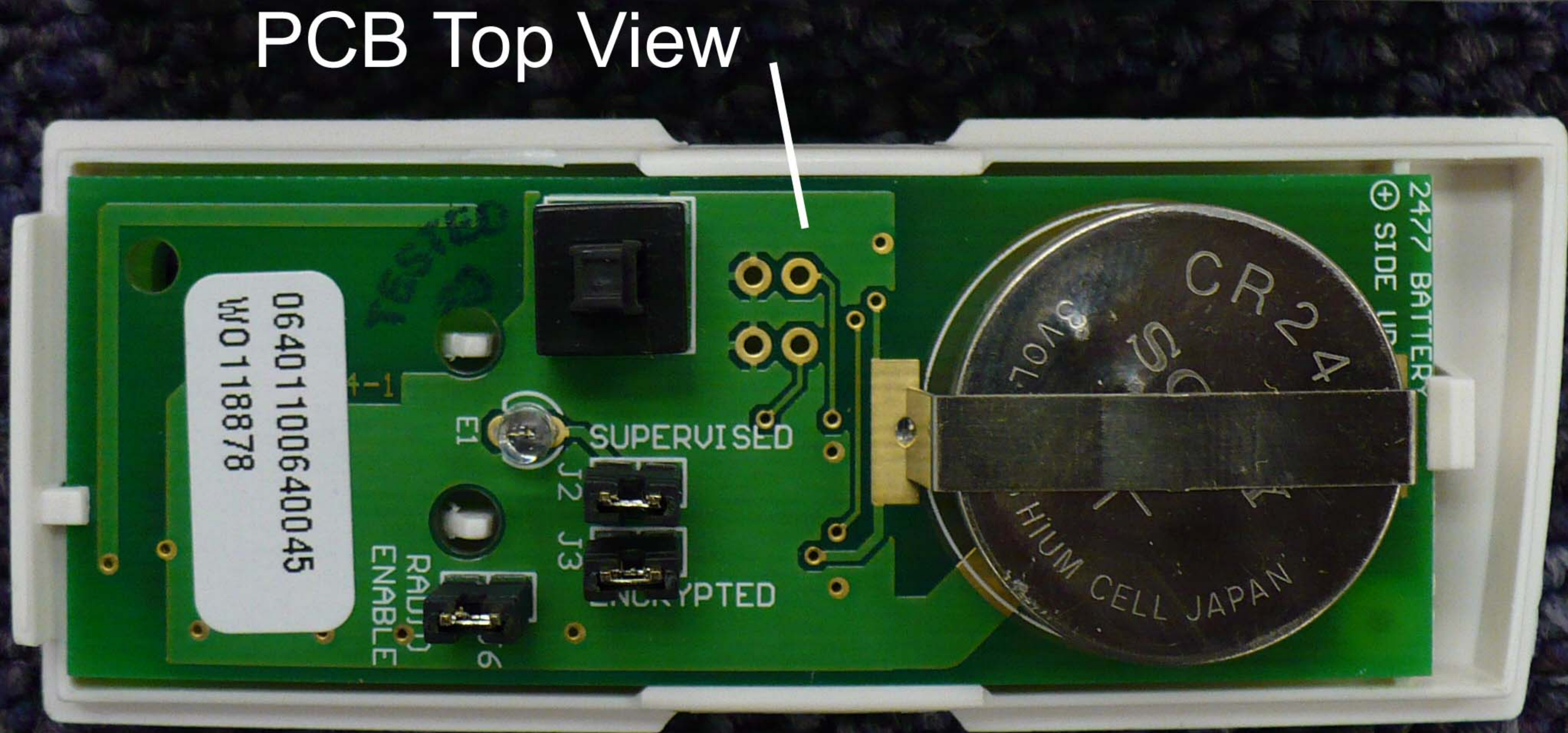
106064 RR1 Wireless Reed Switch Transmitter Inside View
