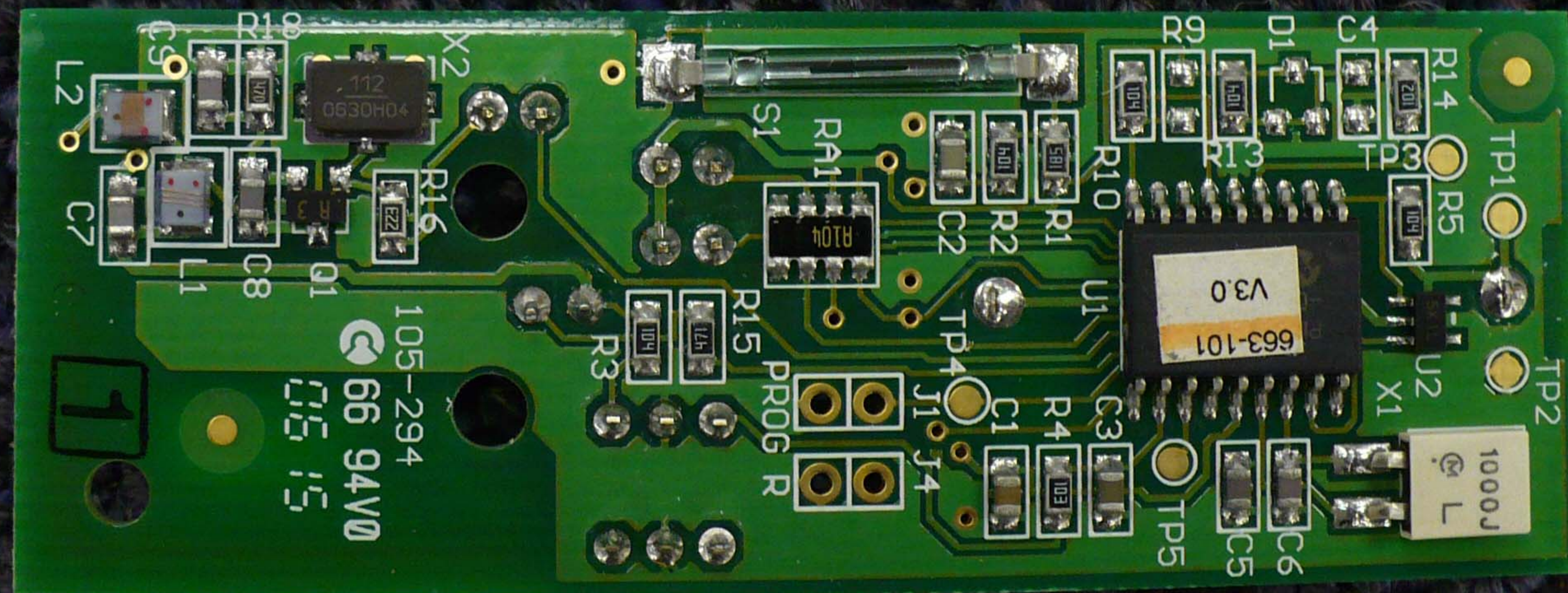
106064 RR1 Wireless Reed Switch Transmitter PCB Back View
