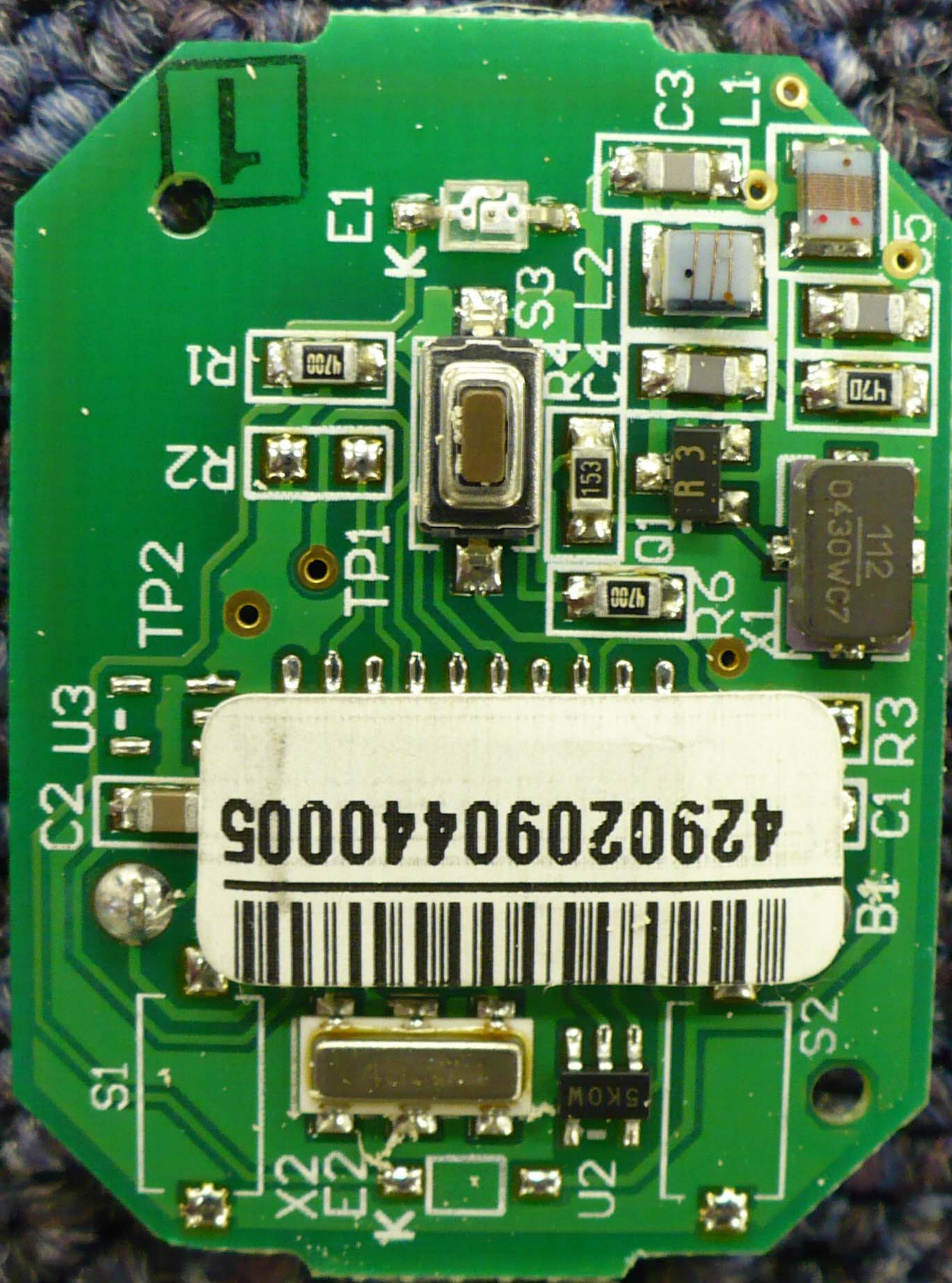
106-050 RK1 Wireless Key Pendant Transmitter PCB Front View
