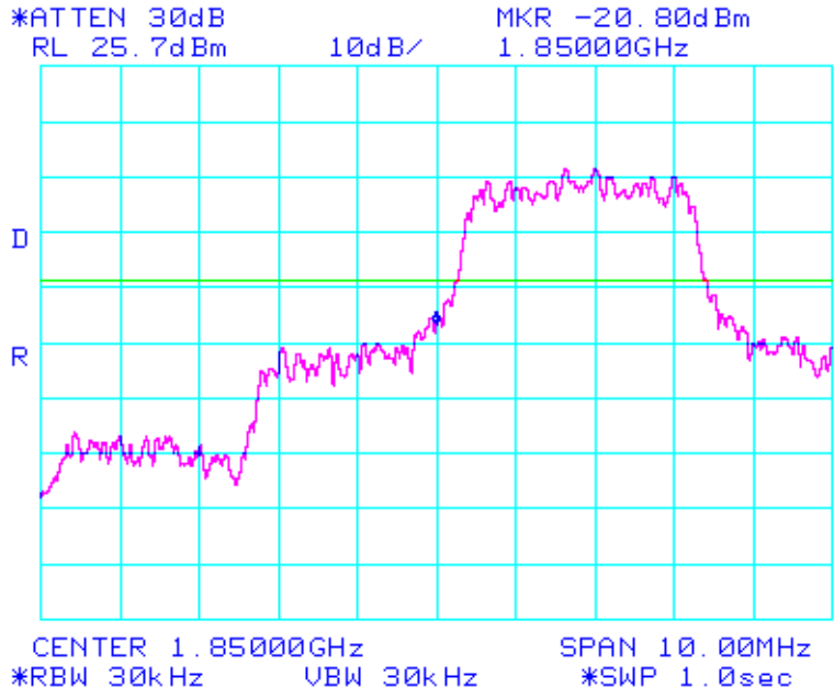
Spur emissions at frequency blockedge +/- 1MHz. Low side of A block emi1298
