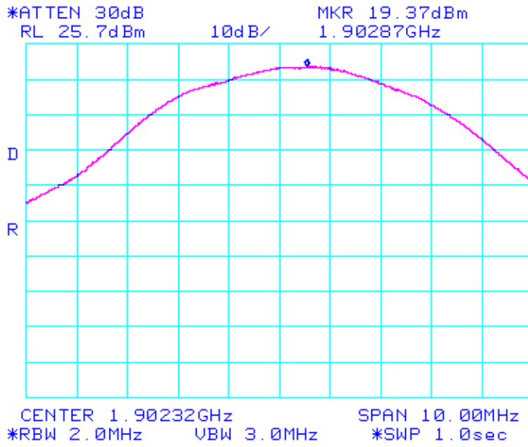
RF power output at antenna terminal. C block (ST) emi1298
