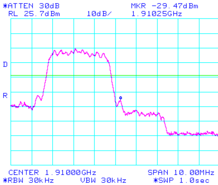
Spur emissions at frequency blockedge +/- 1 MHz. Hi side of C block emi1298
