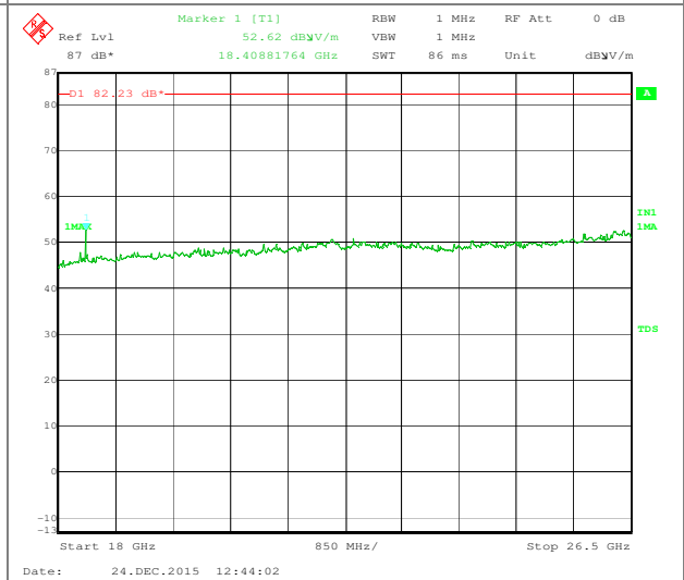
18 - 26 GHz, V: Upper band worst case
