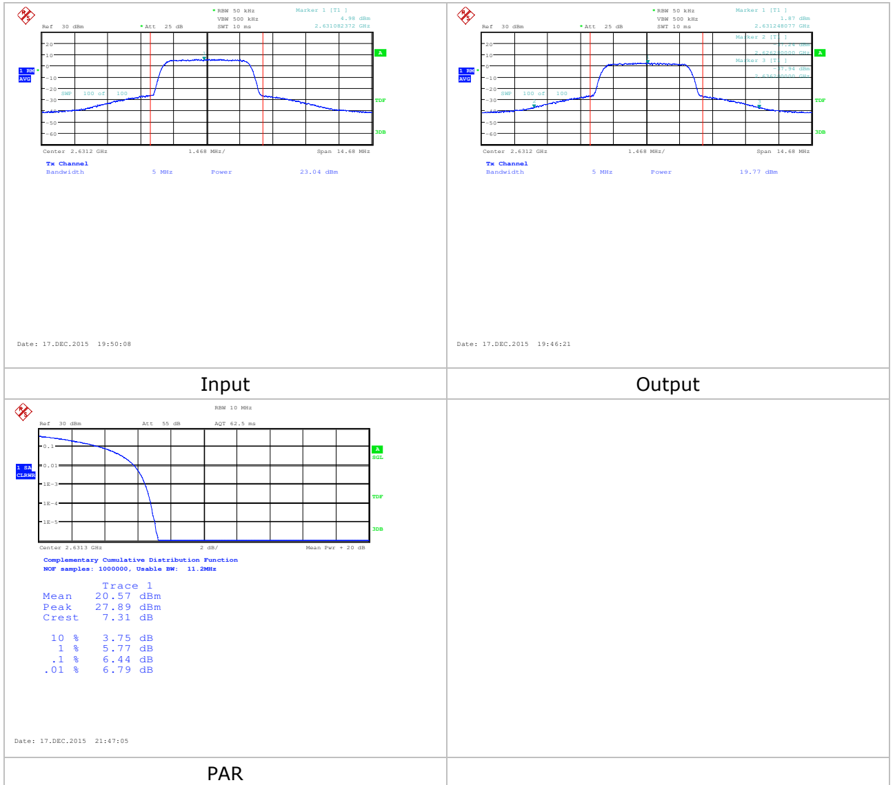
Figure 6: Power and Peak to Average (PAR) plots; 2620-2690 MHz band
