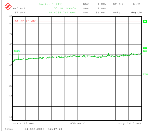
18 - 26 GHz, H: Upper band worst case
