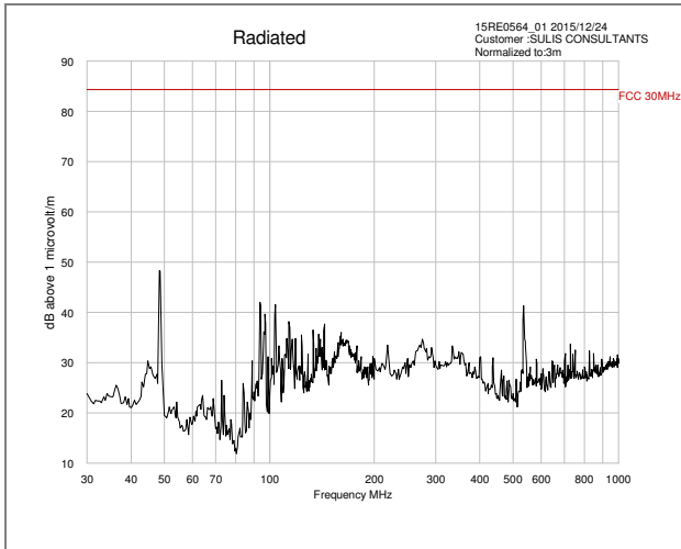
30 – 1000 MHz: both bands
