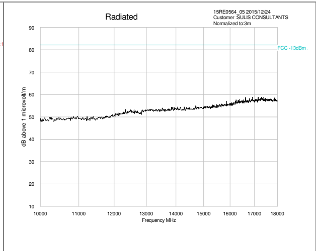
10 – 18 GHz: Upper band worst case
