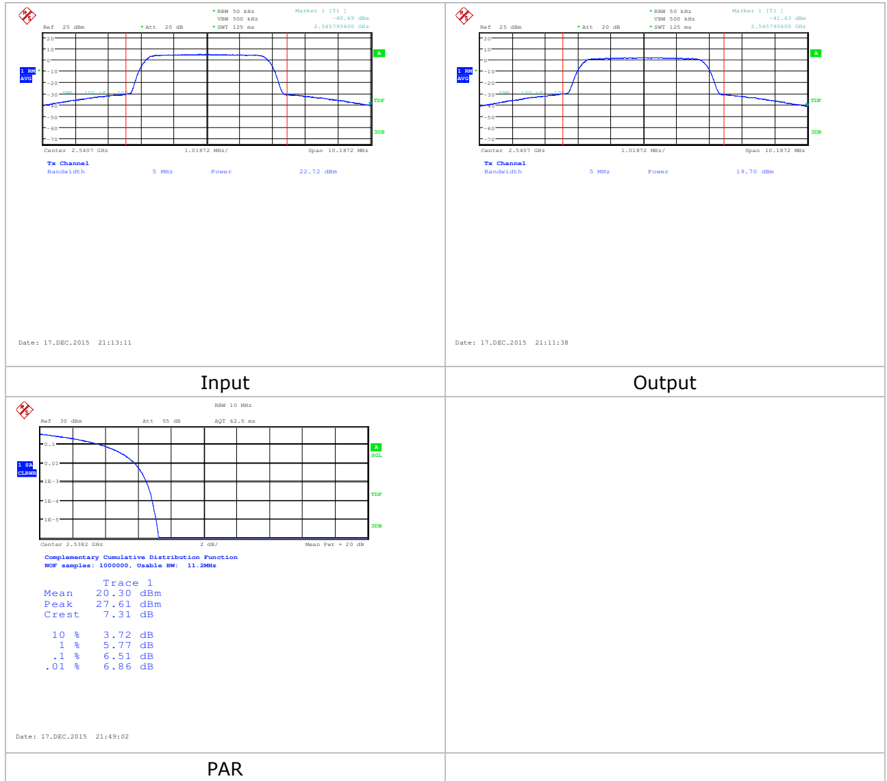
Figure 5: Power and Peak to Average (PAR) plots; 2500-2570 MHz band
