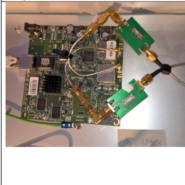
Main PCB and filter PCBs
