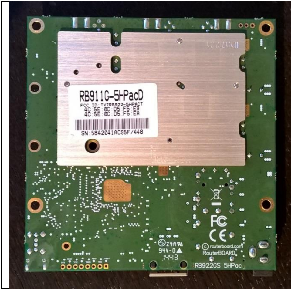
Bottom of PCB
