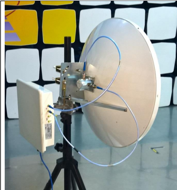
iB440 with external 28.6 dBi antenna (cables connected to the "IB" ports)
