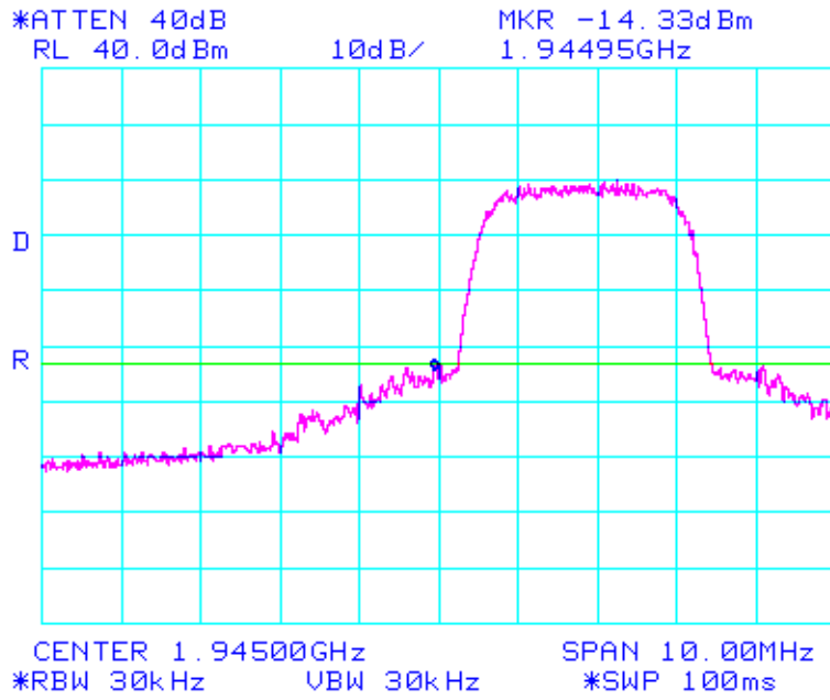
Conducted spur emissions at frequency blockedge +/- 1MHz at Low side of D emi1298
