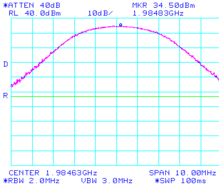
RF power output at antenna terminal block C emi1298
