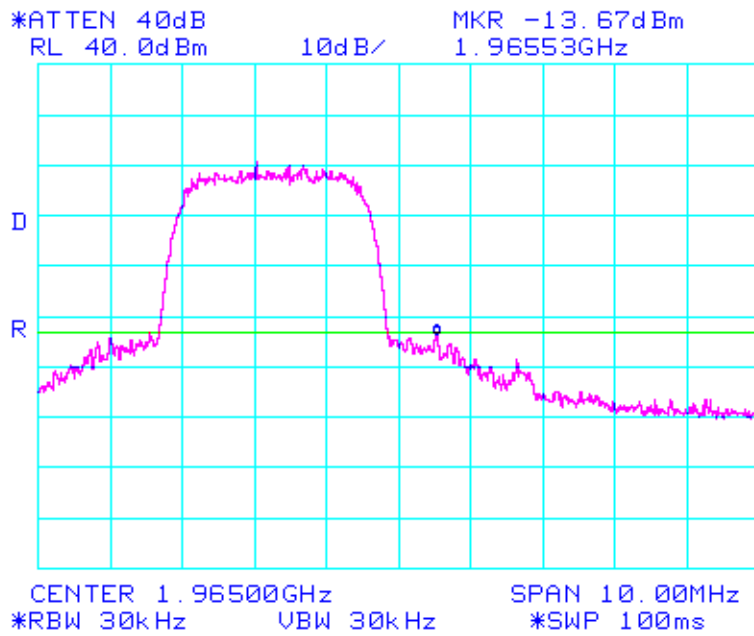
Conducted spur emissions at frequency blockedge +/- 1MHz High side of B emi1298
