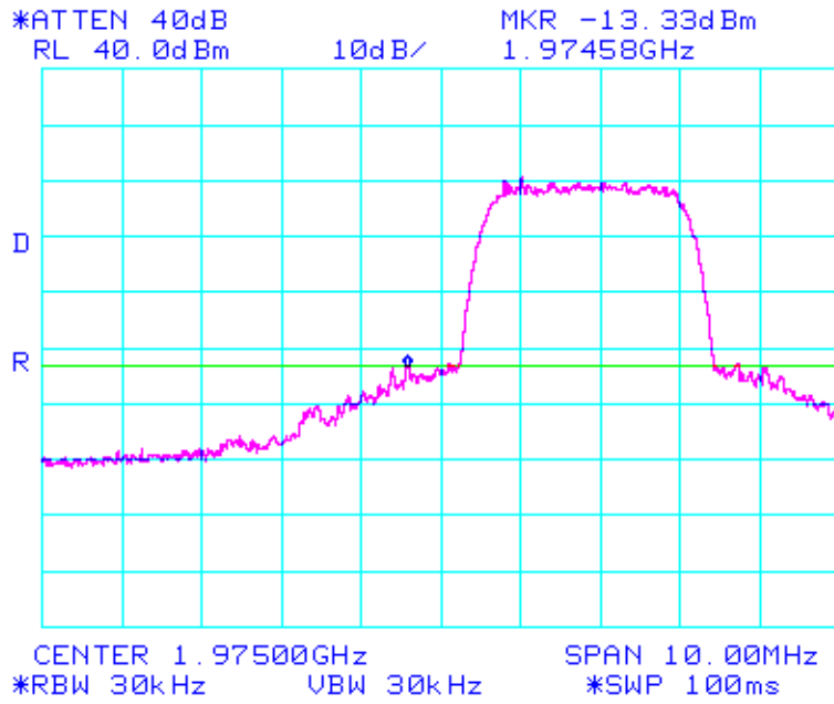
Conducted spur emissions at frequency blockedge +/- 1MHz Low side of block C emi1298
