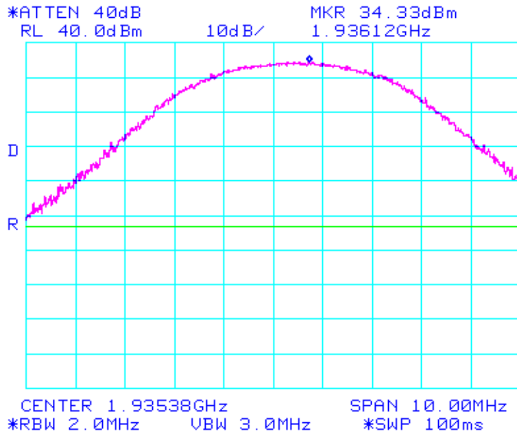
RF power output at antenna terminal block A emi1298
