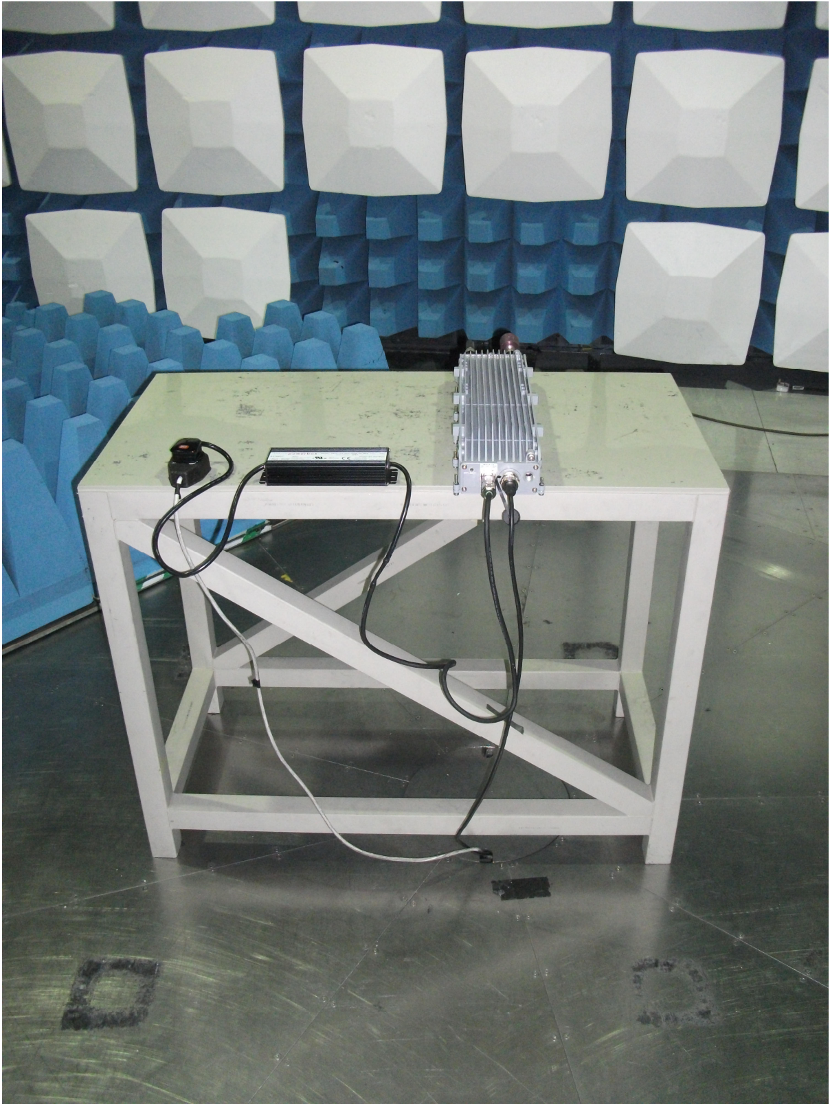
Radiated Spurious Emissions
