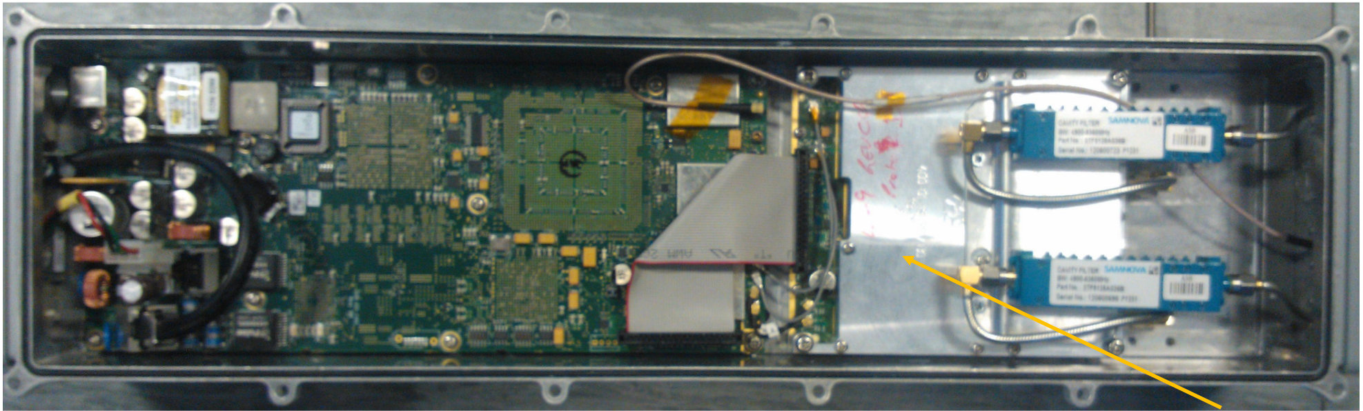
RF FEM with can fitted
