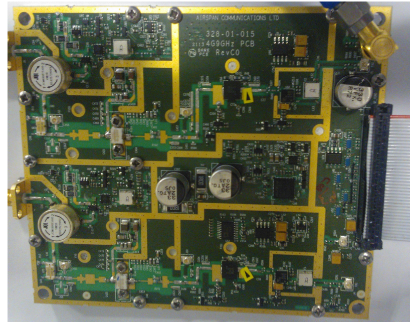
RF FEM without can
