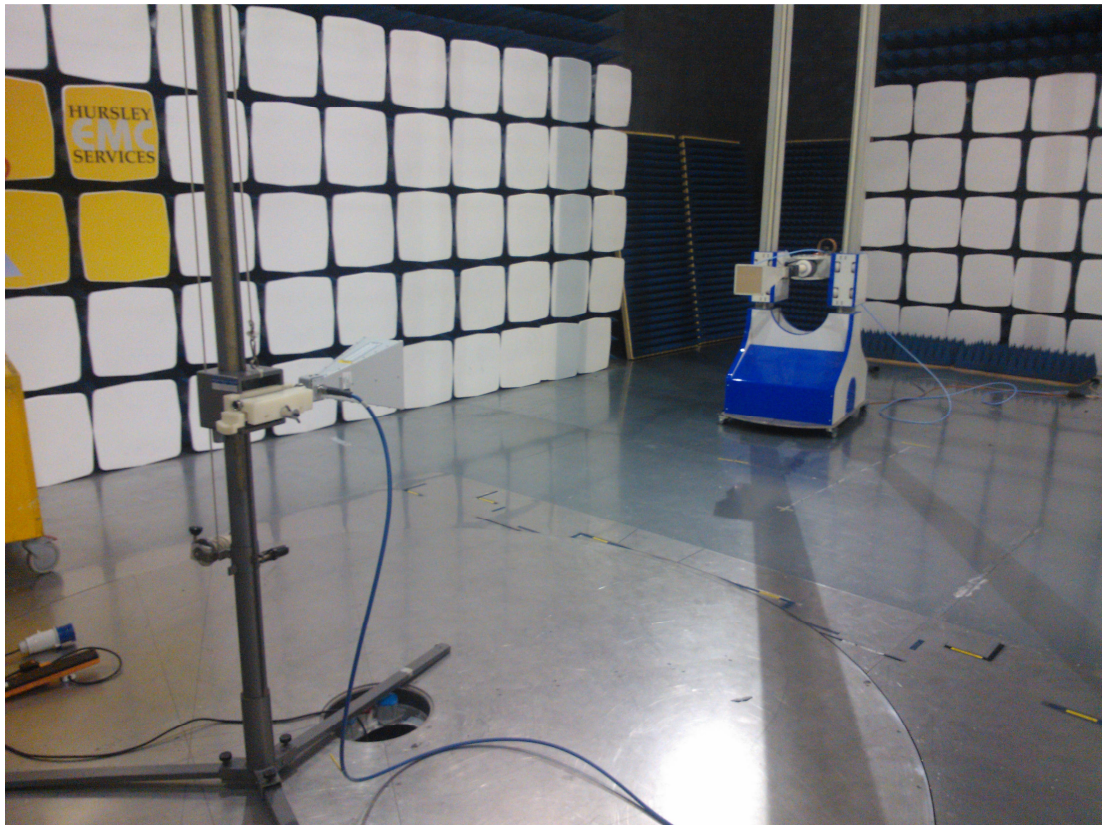
Substitution measurement
