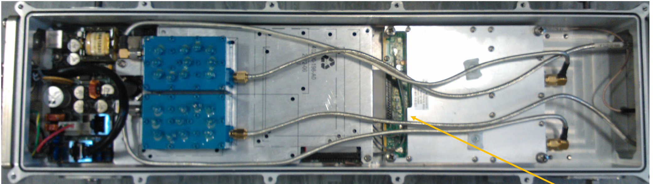
RF FEM with can fitted
