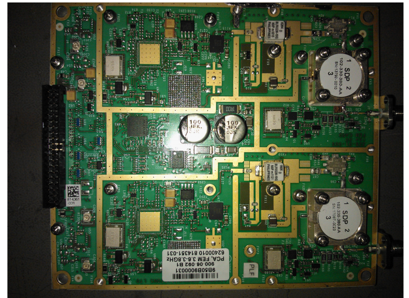
RF FEM without can
