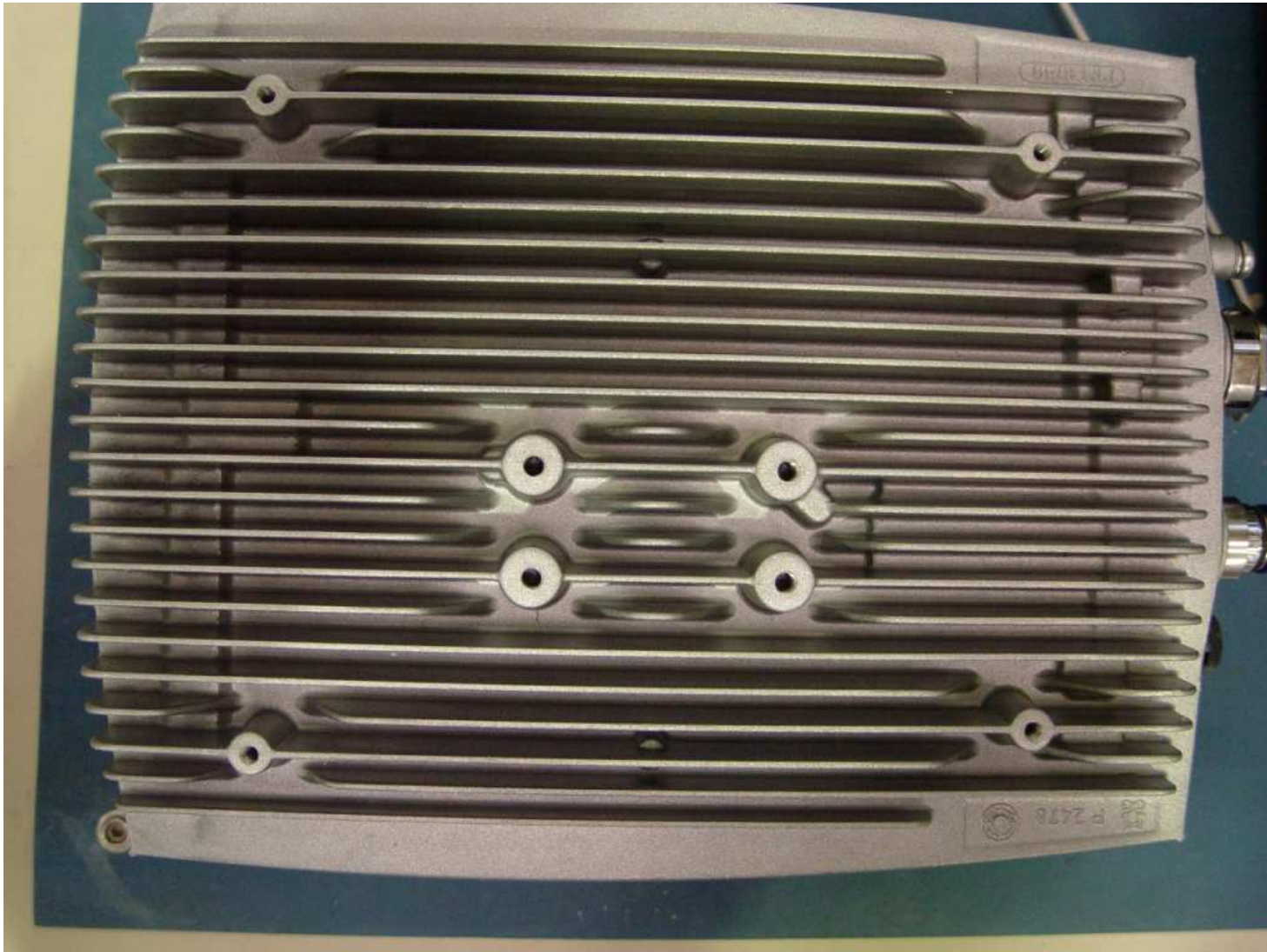
Rear face of SCR showing mounting holes
