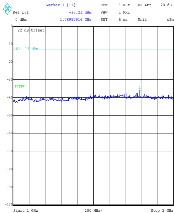
Title: 49355JD02 FCC PART 90 Comment A: TX CONDUCTED EMISSIONS 10 MHz TOP CHANNEL Date: 6.AUG.2007 15:14:41
