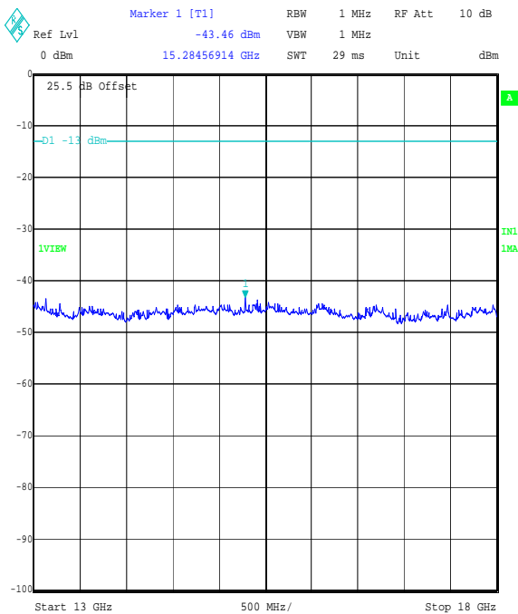
Title: 49355JD02 FCC PART 90 Comment A: TX CONDUCTED EMISSIONS 10 MHz TOP CHANNEL Date: 6.AUG.2007 15:23:33
