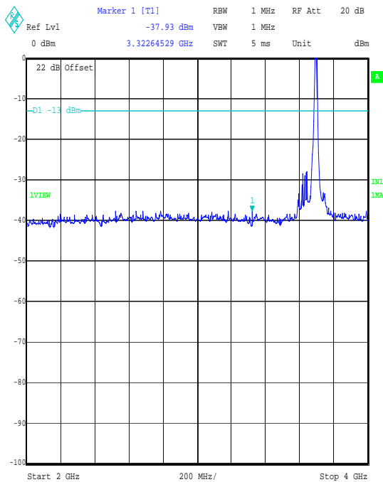
Title: 49355JD02 FCC PART 90 Comment A: TX CONDUCTED EMISSIONS 10 MHz TOP CHANNEL Date: 6.AUG.2007 15:16:17
