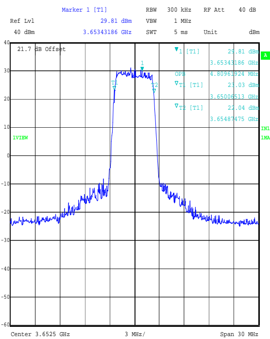
Title: 49355JD02 FCC PART 90 Comment A: OCCUPIED BANDWIDTH 5 MHz BOTTOM CHANNEL Date: 24.JUL.2007 15:00:58
