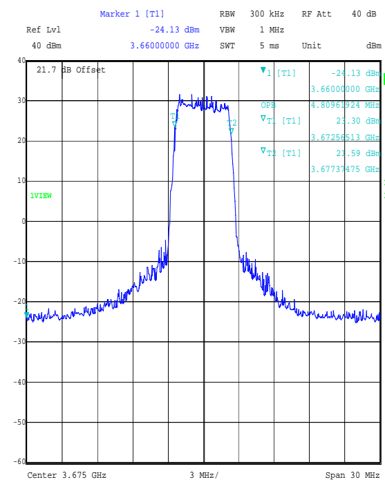
Title: 49355JD02 FCC PART 90 Comment A: OCCUPIED BANDWIDTH 5 MHz CENTRE CHANNEL Date: 24.JUL.2007 15:01:46
