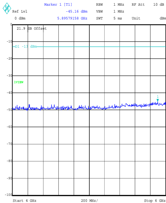
Title: 49355JD02 FCC PART 90 Comment A: TX CONDUCTED EMISSIONS 10 MHz TOP CHANNEL Date: 6.AUG.2007 15:18:01
