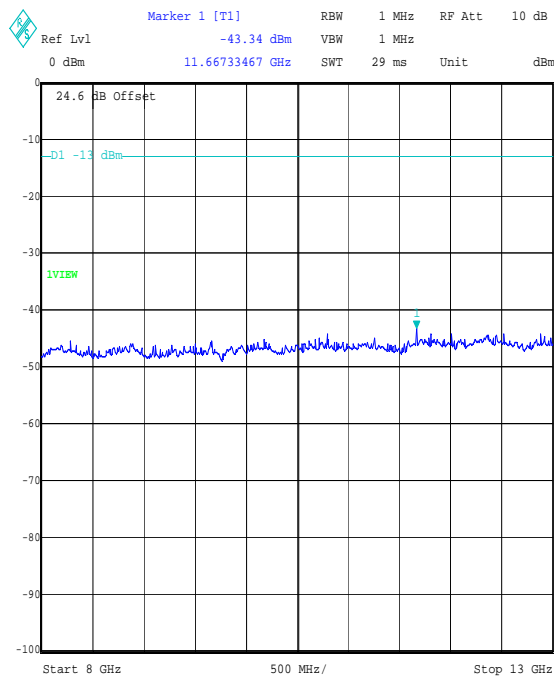
Title: 49355JD02 FCC PART 90 Comment A: TX CONDUCTED EMISSIONS 10 MHz TOP CHANNEL Date: 6.AUG.2007 15:22:32
