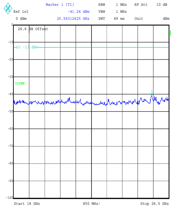
Title: 49355JD02 FCC PART 90 Comment A: TX CONDUCTED EMISSIONS 10 MHz TOP CHANNEL Date: 6.AUG.2007 15:24:52
