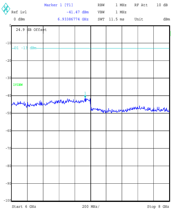
Title: 49355JD02 FCC PART 90 Comment A: TX CONDUCTED EMISSIONS 10 MHz TOP CHANNEL Date: 6.AUG.2007 15:21:15
