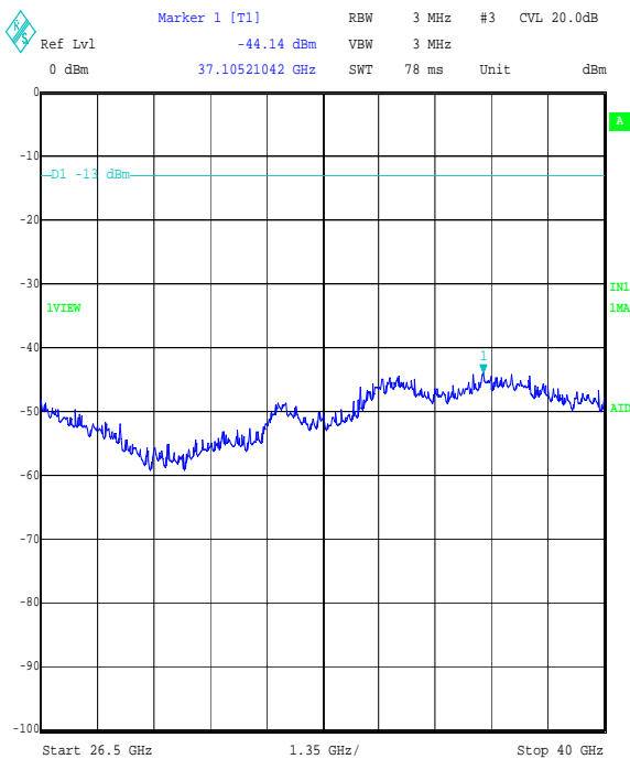
Title: 49355JD02 FCC PART 90 Comment A: TX CONDUCTED EMISSIONS 10 MHz TOP CHANNEL Date: 8.AUG.2007 09:58:41
