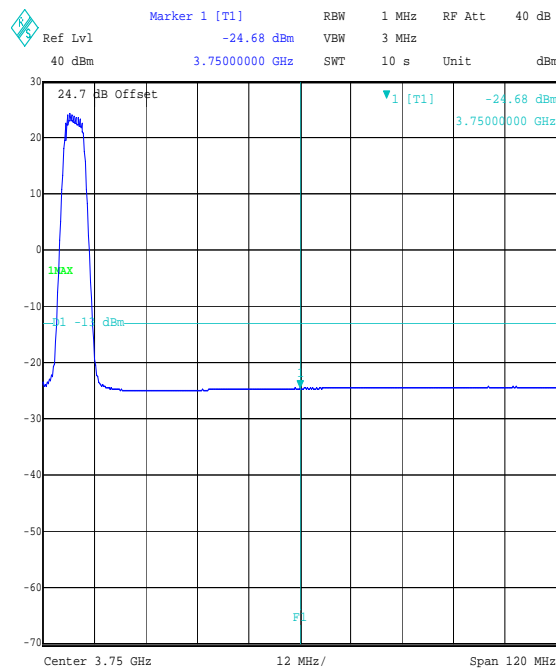
Title: 49355JD02 FCC PART 90 Comment A: CONDUCTED EMISSIONS UPPER BAND EDGE 5 MHz TOP CHANNEL Date: 8.AUG.2007 15:27:09
