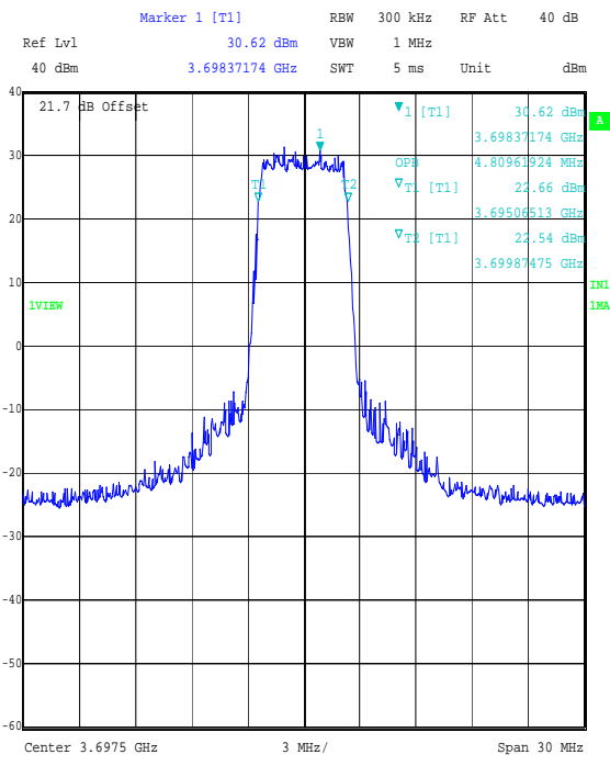
Title: 49355JD02 FCC PART 90 Comment A: OCCUPIED BANDWIDTH 5 MHz TOP CHANNEL Date: 24.JUL.2007 15:02:57
