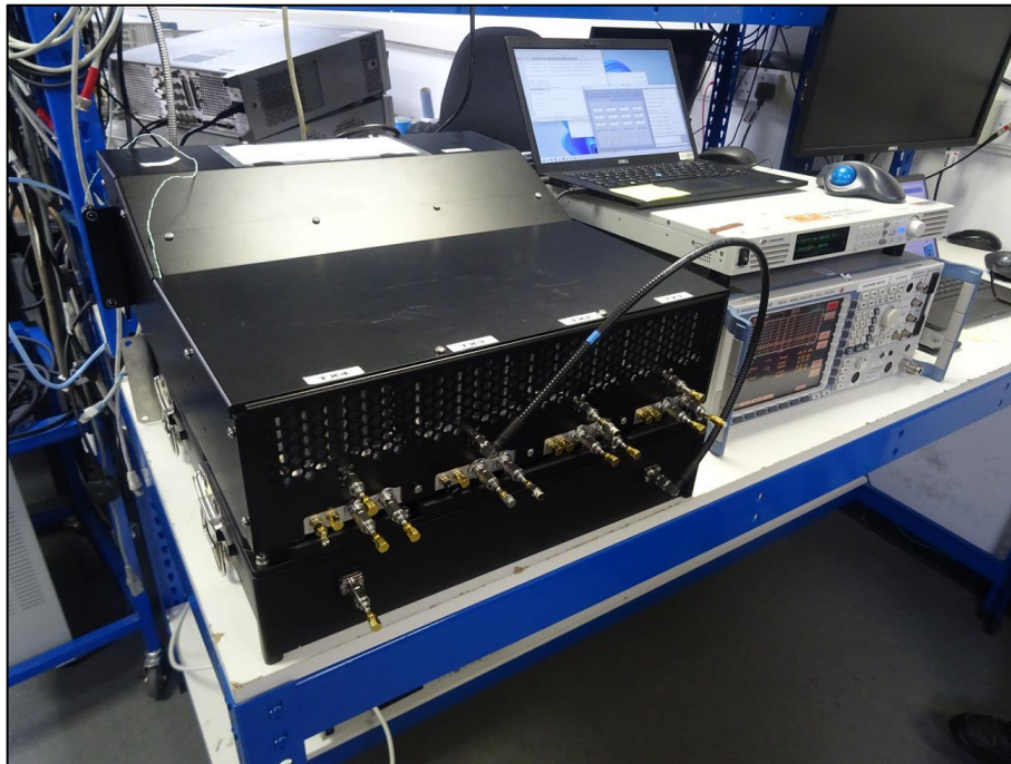
Figure 3 – Conducted Measurements Setup
