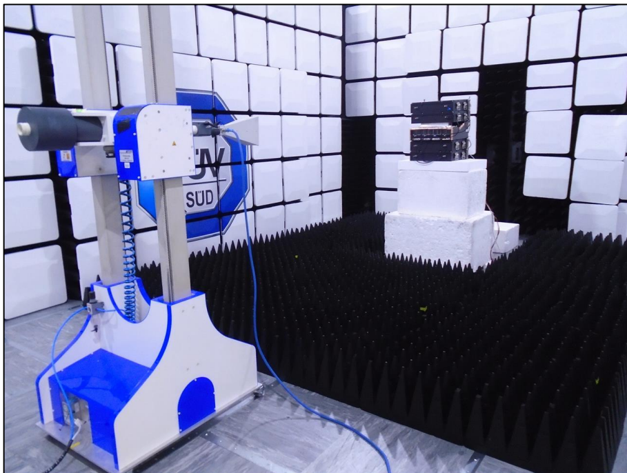
Figure 2 – Radiated Disturbance - 1 GHz to 9 GHz
