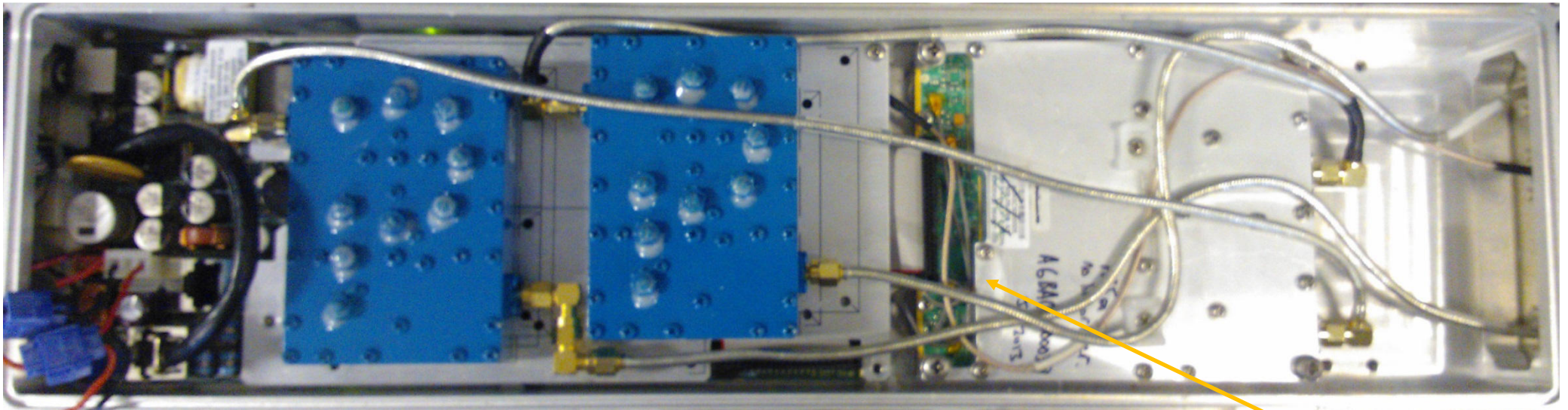
RF FEM with can fitted
