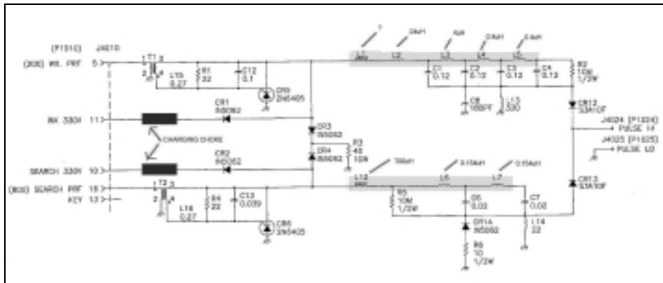
Figure 1-1 Modulator Schematic
