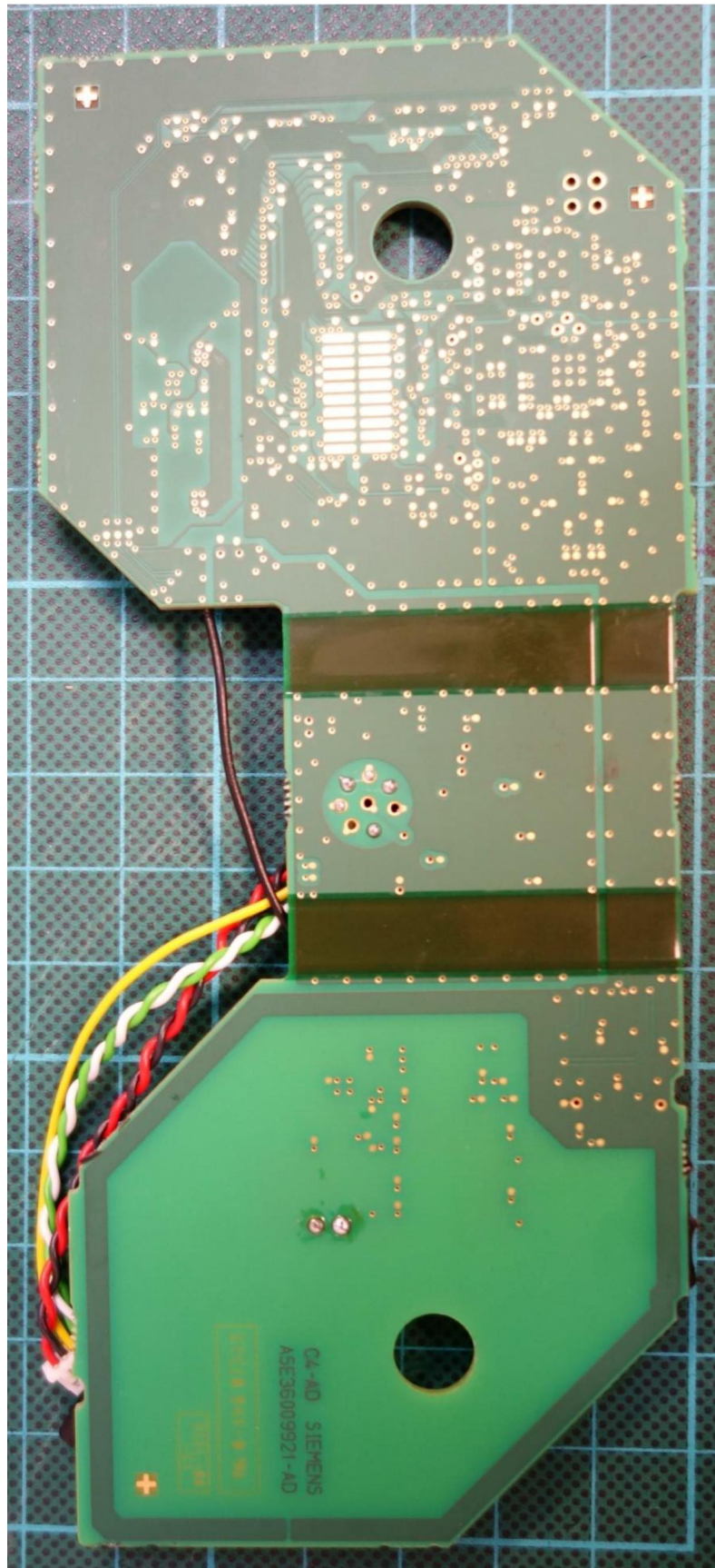
80014371 Siemens Simatic RF350R-Reader – bottom view
