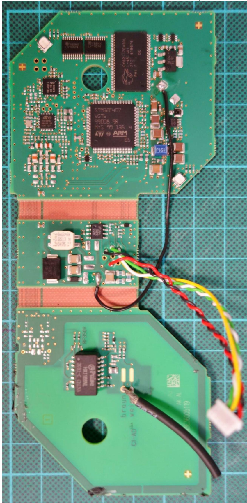
80014371 Siemens Simatic RF350R-Reader – top view
