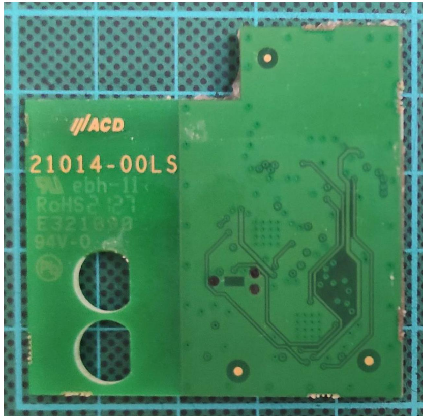
80014318 ACD M2Smart RFID HF Siemens Mainboard – bottom view
