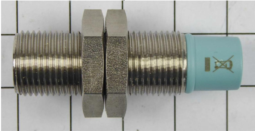
ANT 12 metal (6GT2398-1DC00) Top view
