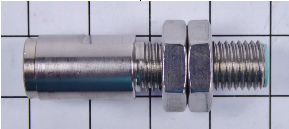
ANT 8 (6GT2398-1CF00) Top view
