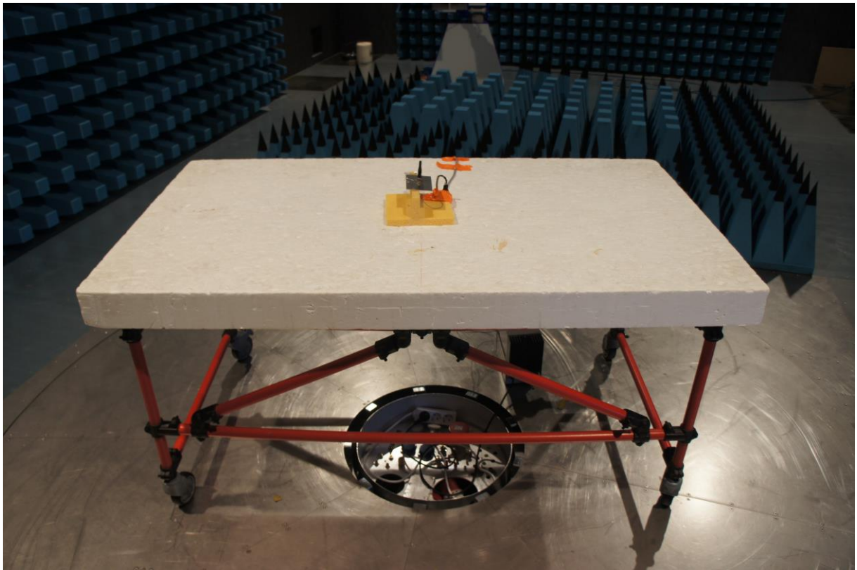
Picture 14: EUT test setup radiated emissions > 1GHz - front view
