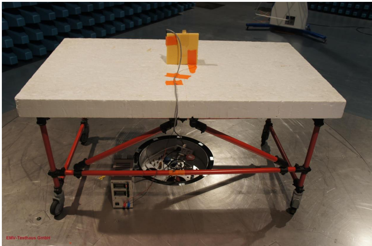
Picture 12: test setup radiated emissions 30 MHz - 1 GHz, rear view
