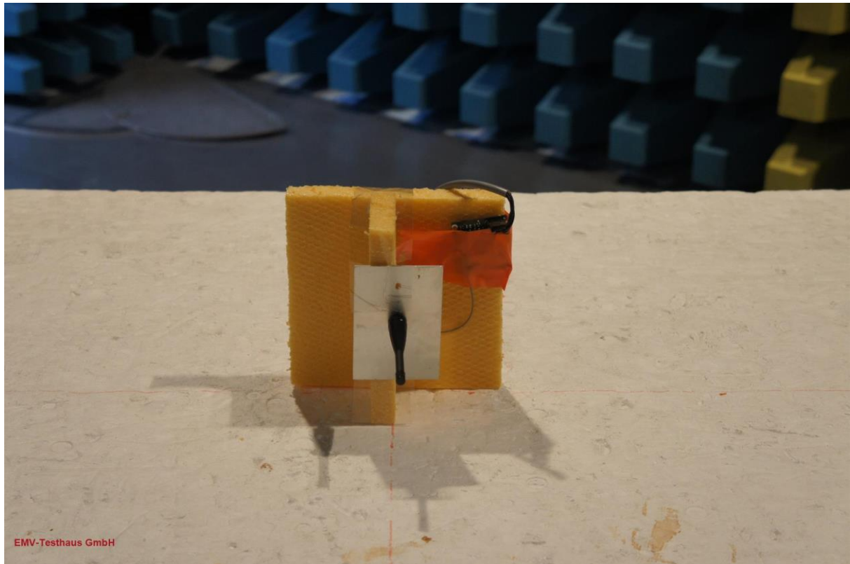
Picture 11: test setup radiated emissions 30 MHz - 1 GHz, front view
