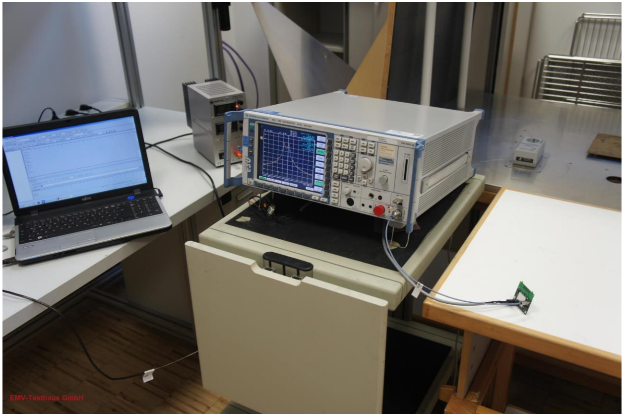
Picture 13: EUT test setup conducted measurements
