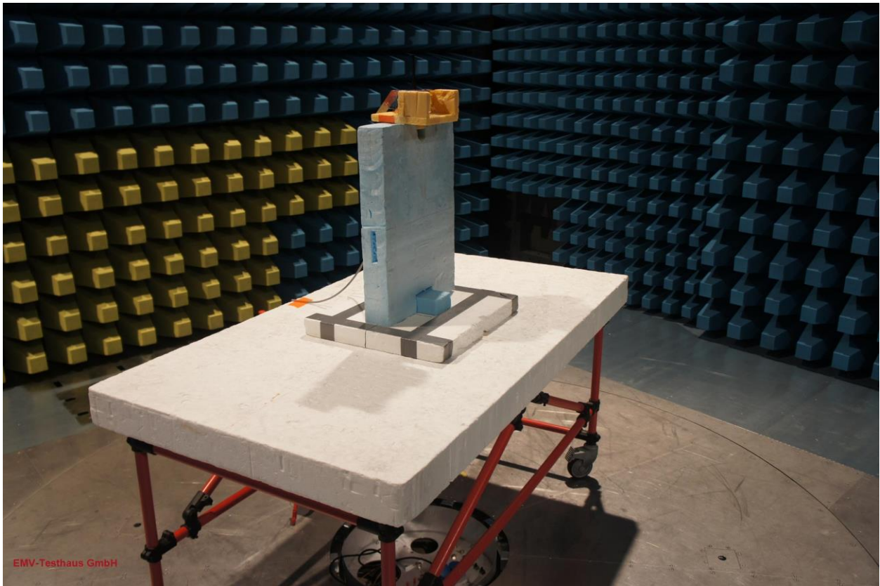
Picture 6: test setup “transmitter rad. field strenght”, “band-edge compliance”
