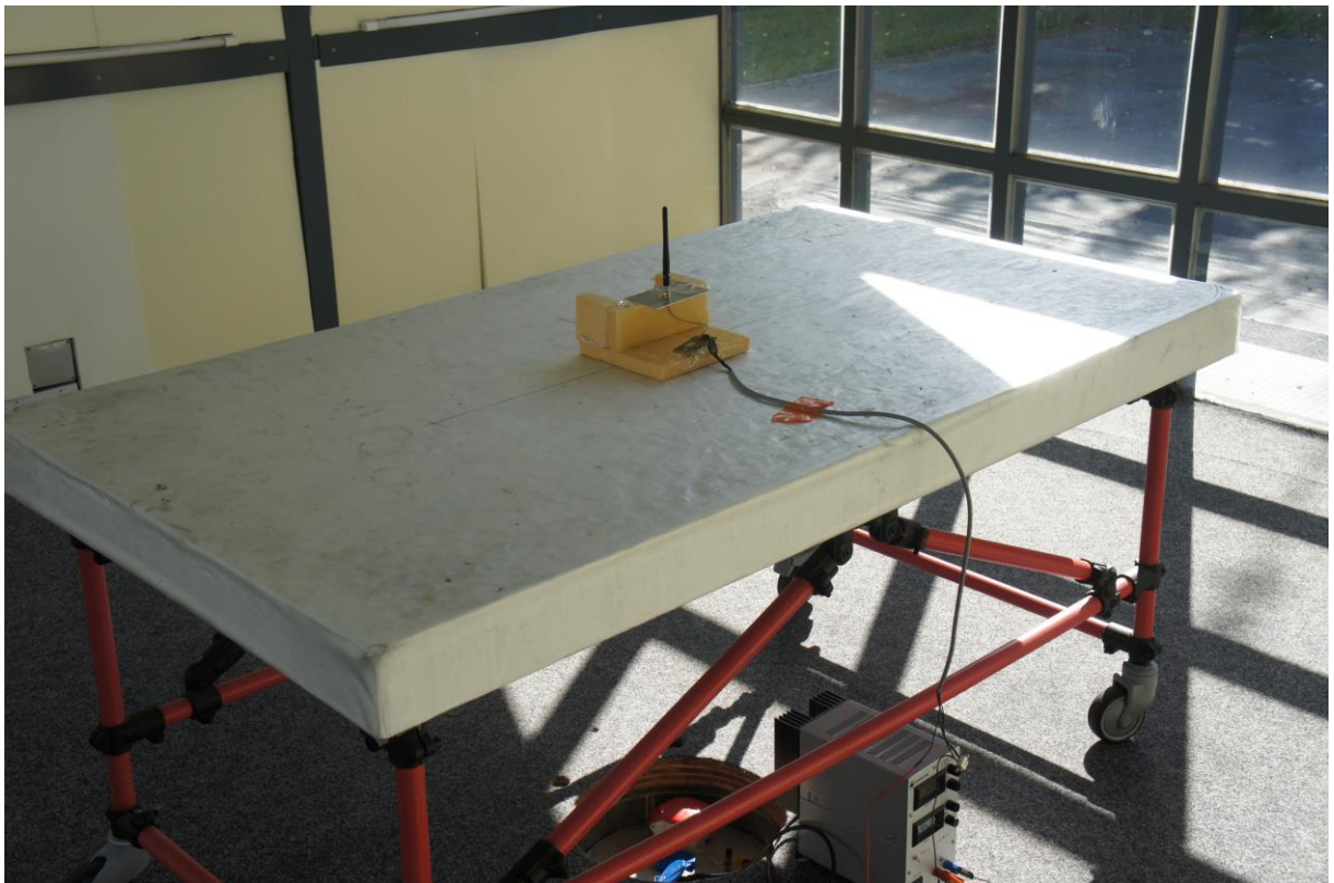
Picture 10: test setup radiated emissions 9 kHz - 30 MHz, OATS, rear view
