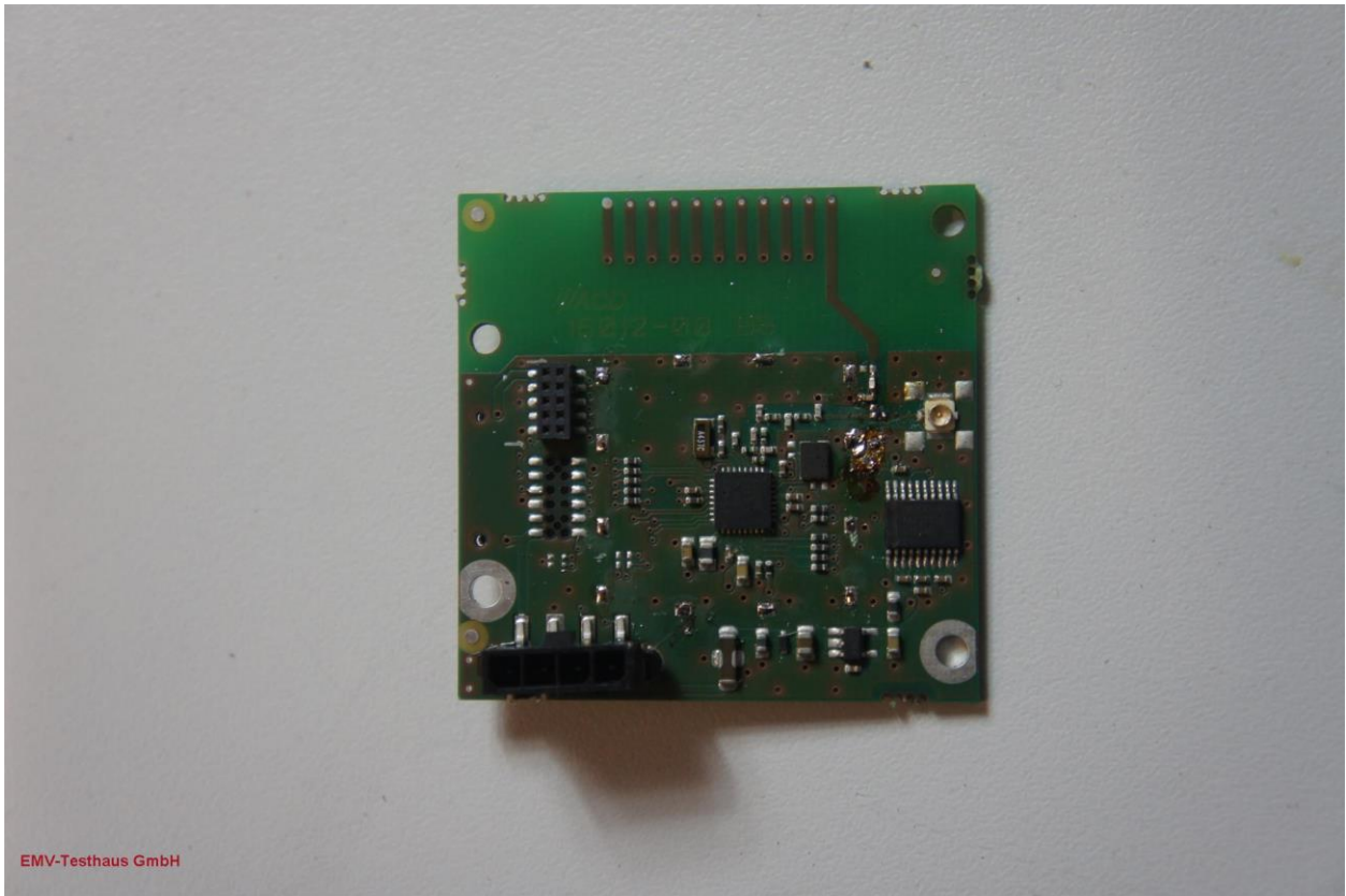
Picture 1: EUT - top side, open RF-shielding
