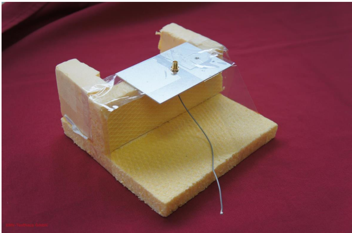
Picture 4: Antenna reference plane
