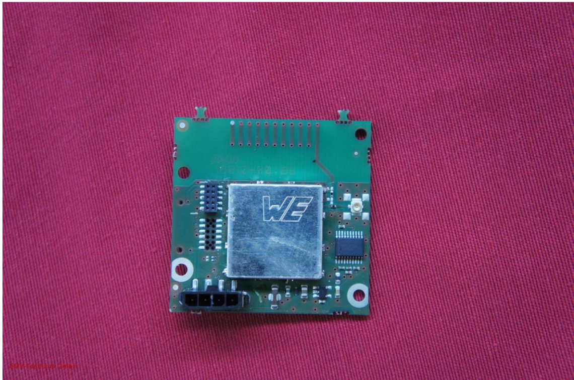
Picture 1: EUT - top side
