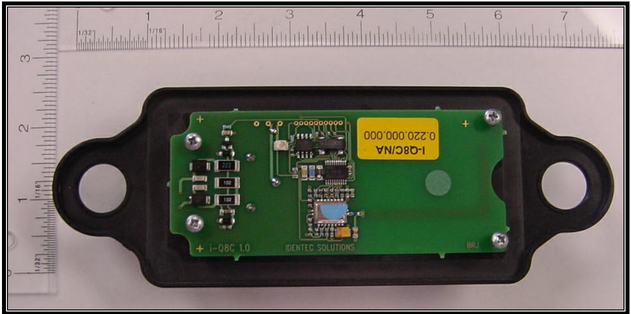
PHOTOGRAPH 9: i-Q8C PCB IN CASE
