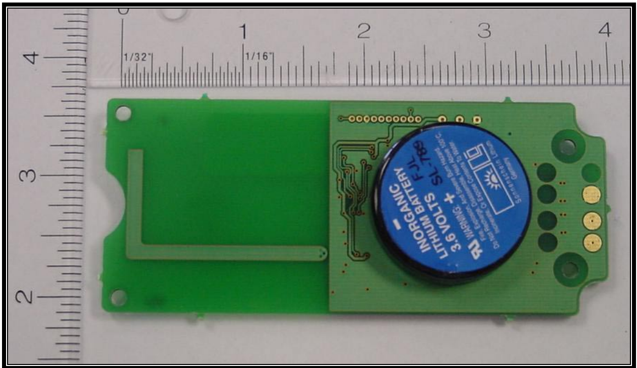
PHOTOGRAPH 12: i-Q8C CIRCUIT CARD BOTTOM
