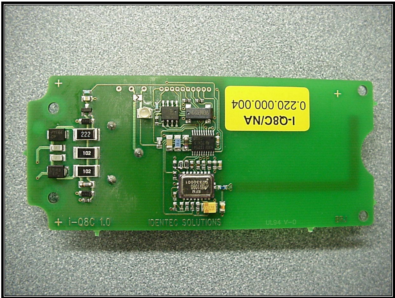
PHOTOGRAPH 11: i-Q8C CIRCUIT CARD TOP
