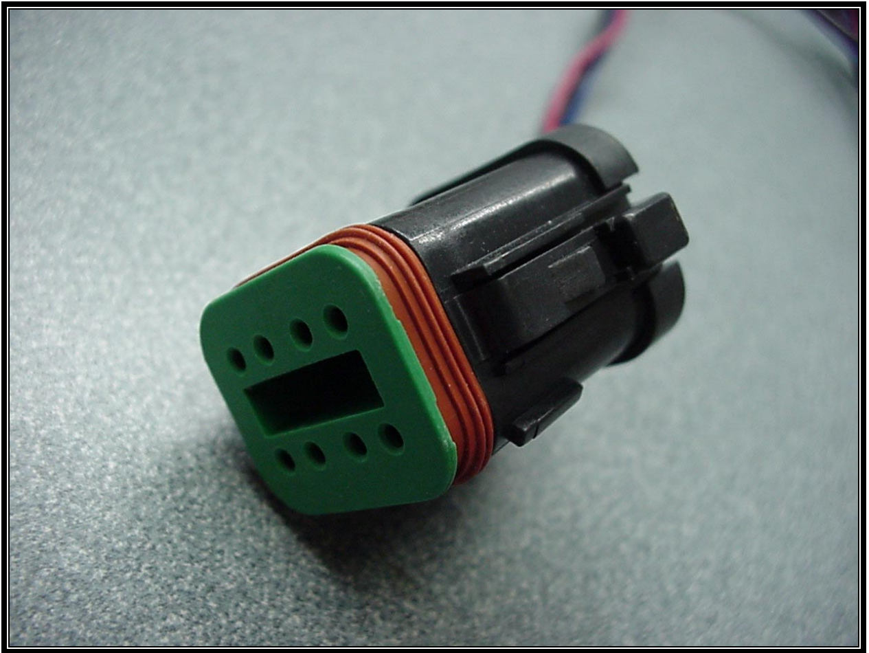
PHOTOGRAPH 8: i-Q8C CONNECTOR
