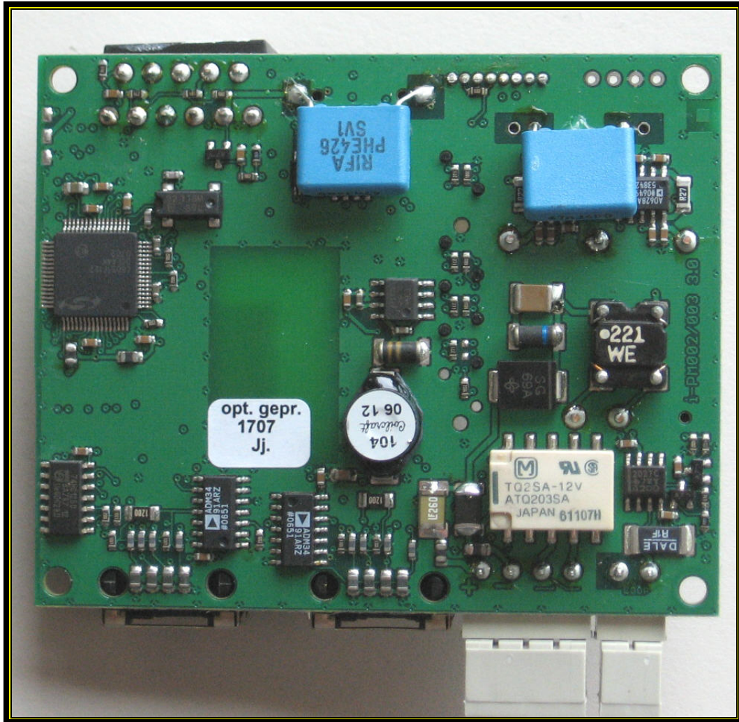
Photograph 10: PCB Bottom View
