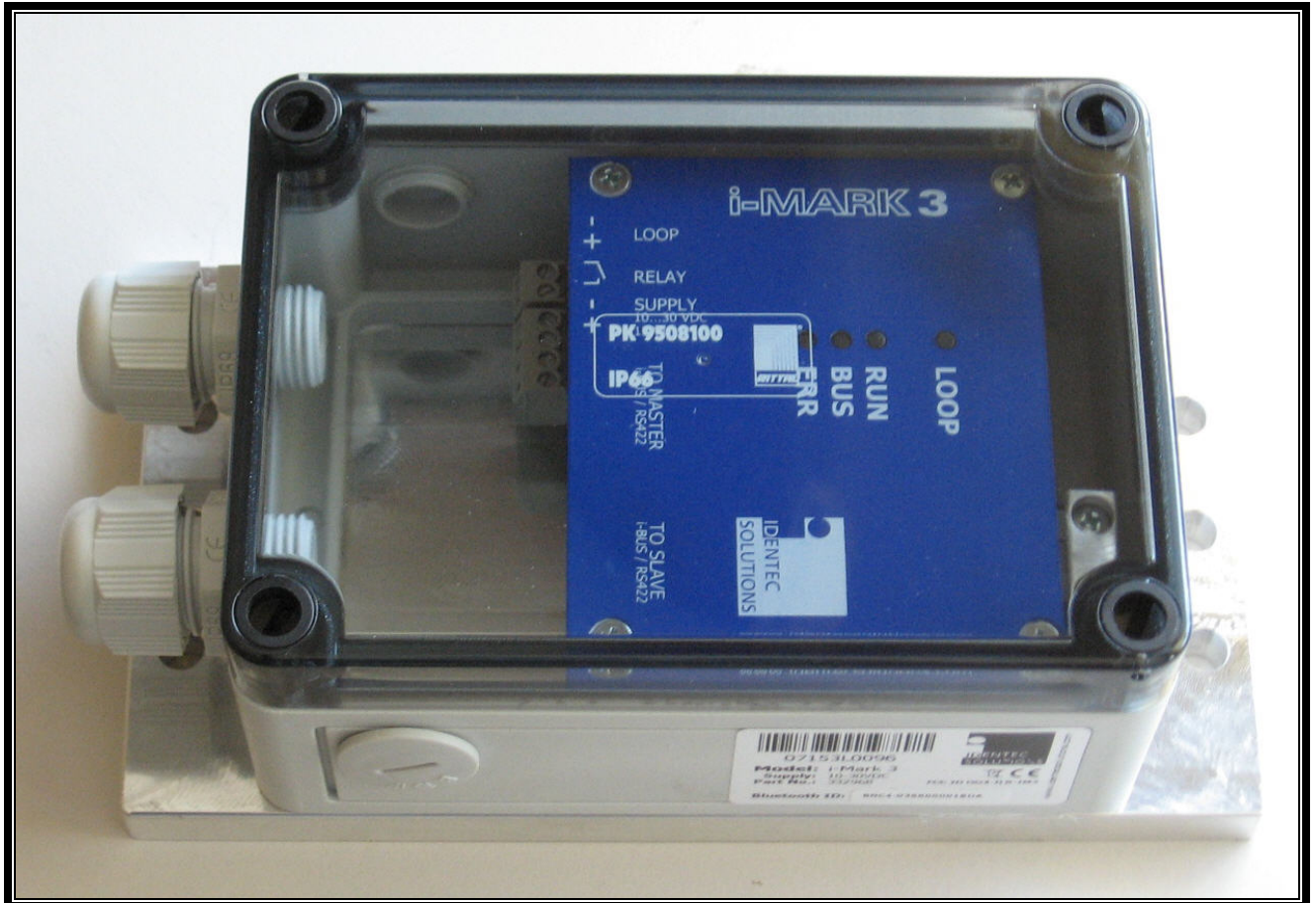
Photograph 8: Side View of EUT
