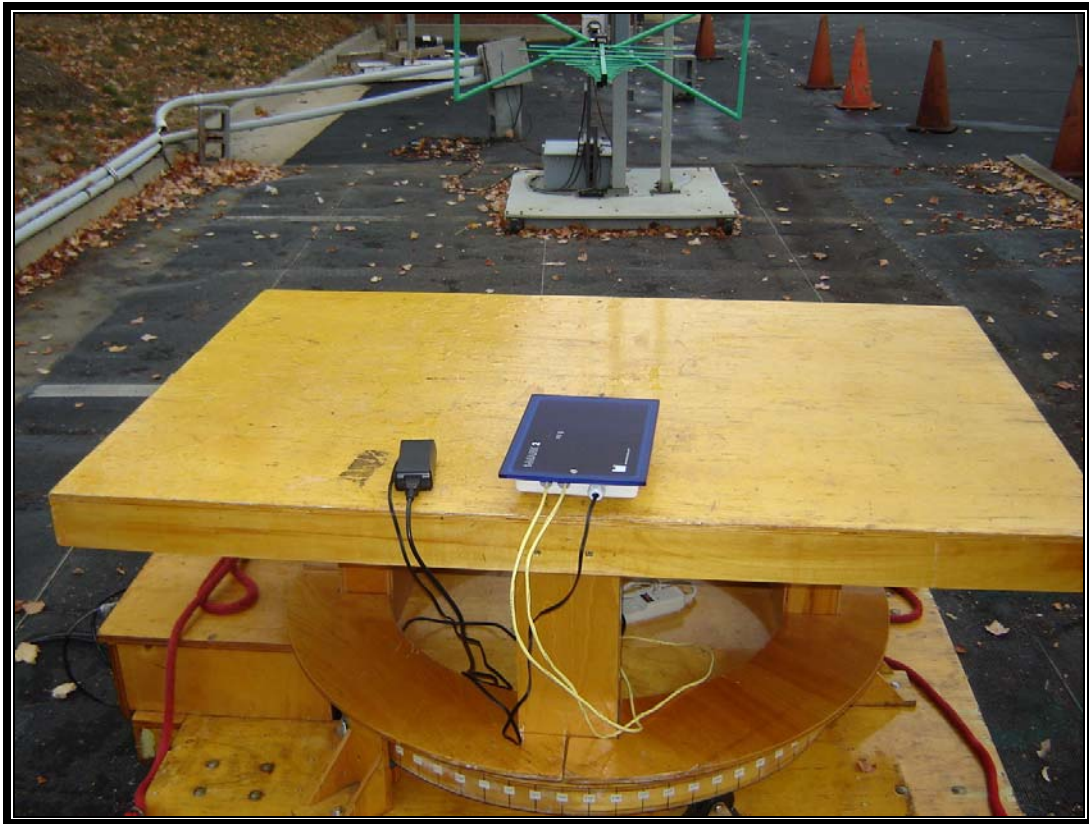
Photograph 4: Radiated Testing – Back View
