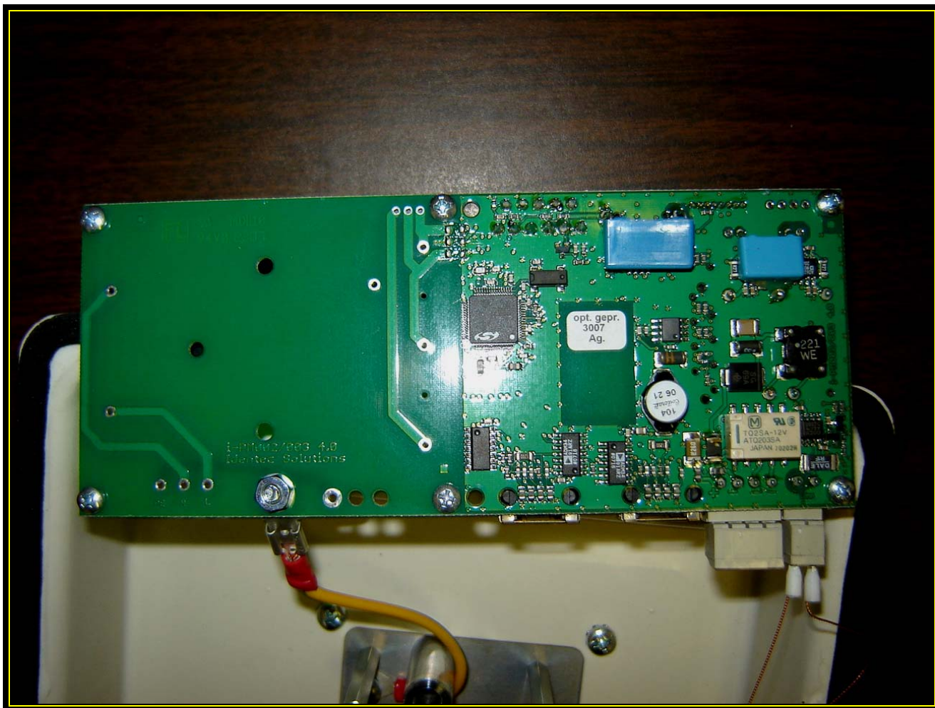
Photograph 10: PCB Bottom View
