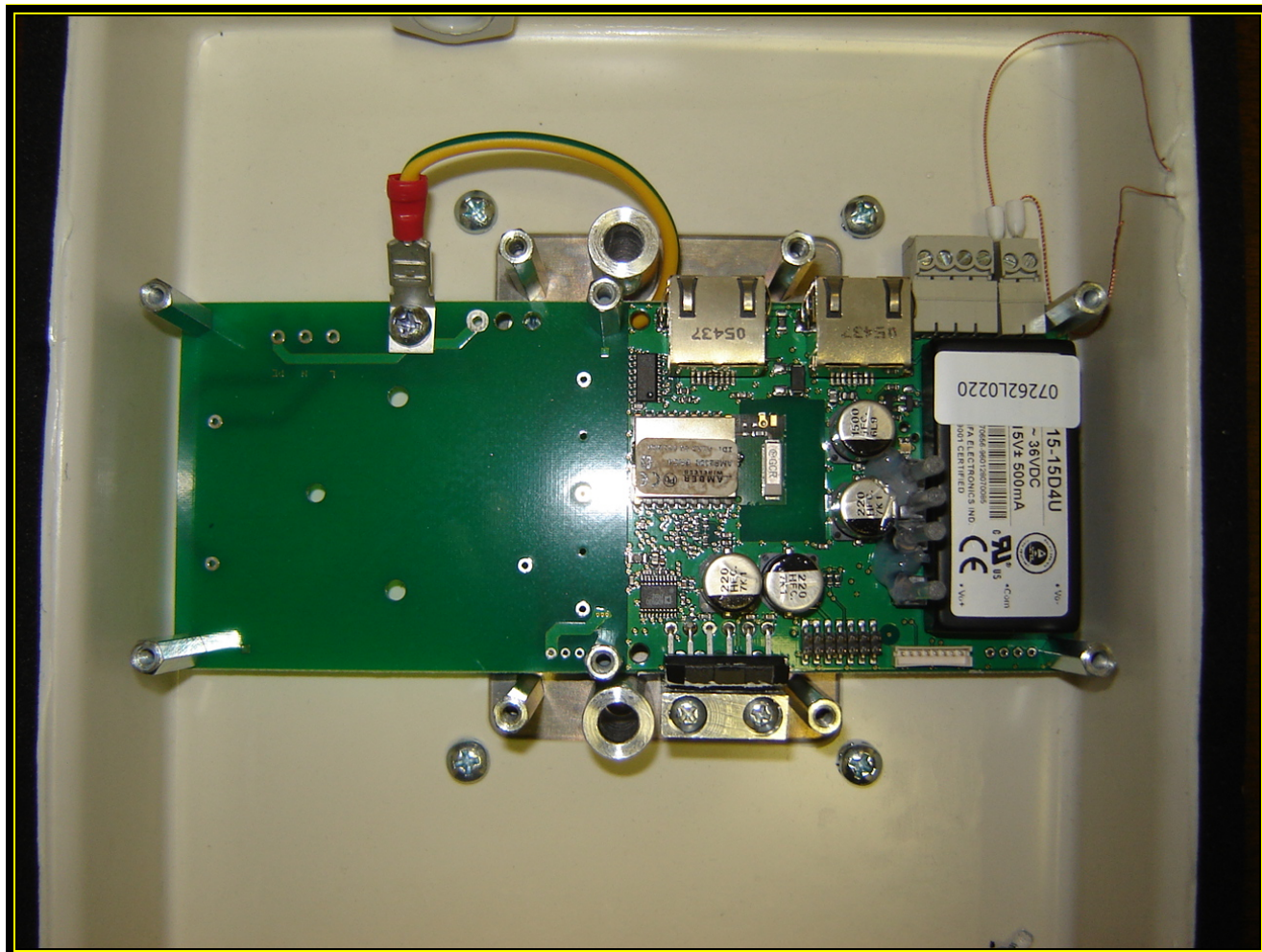
Photograph 8: PCB Top View without Cover in EUT
