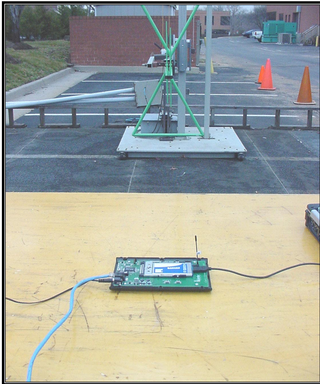
PHOTOGRAPH 2: RADIATED TEST CONFIGURATION ( \frac{1}{4} WAVE WHIP ANTENNA REAR VIEW)
