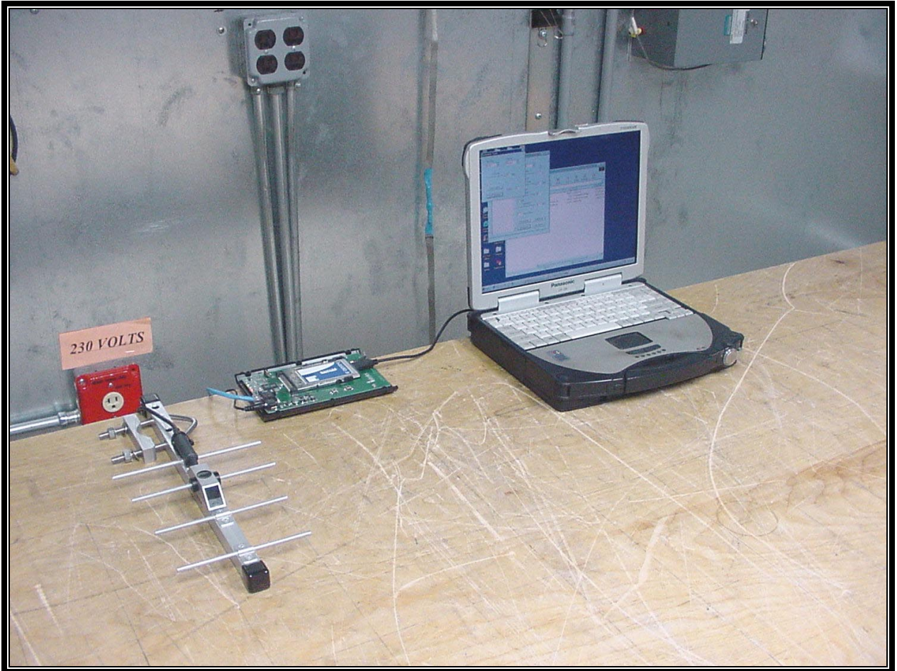
PHOTOGRAPH 15: CONDUCTED TEST CONFIGURATION (YAGI ANTENNA FRONT VIEW)
