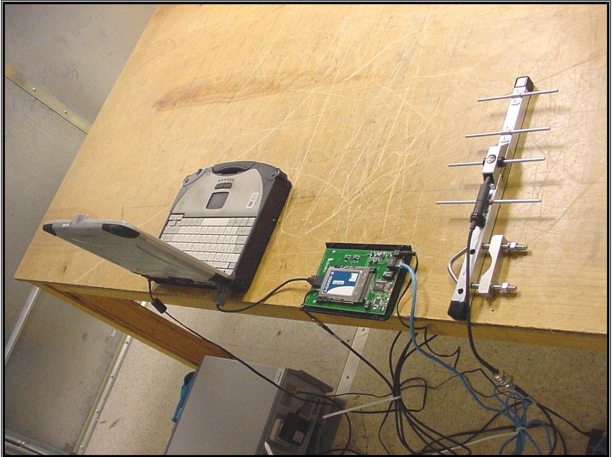
PHOTOGRAPH 16: CONDUCTED TEST CONFIGURATION (YAGI ANTENNA REAR VIEW)
