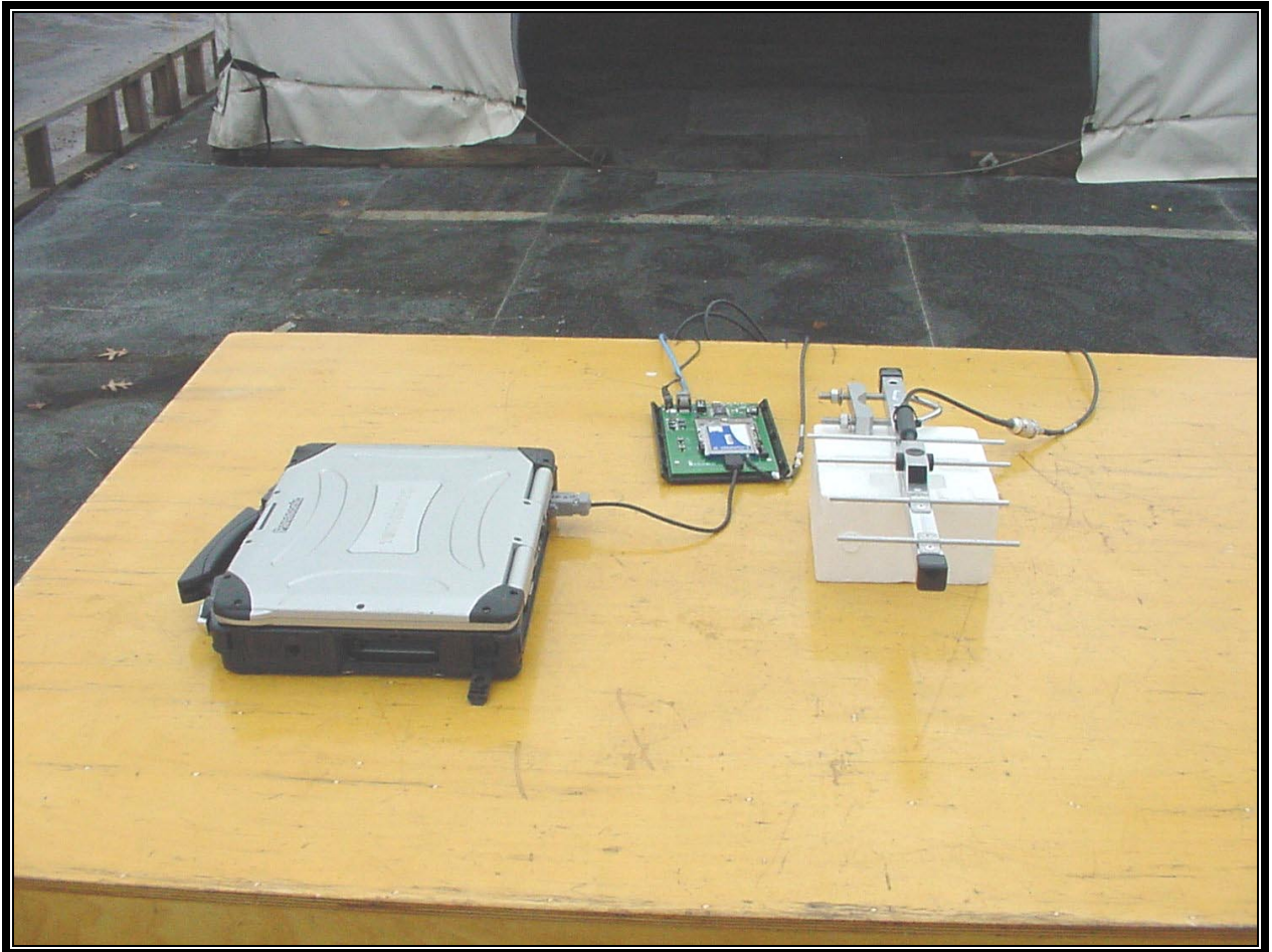
PHOTOGRAPH 7: RADIATED TEST CONFIGURATION (YAGI ANTENNA FRONT VIEW)
