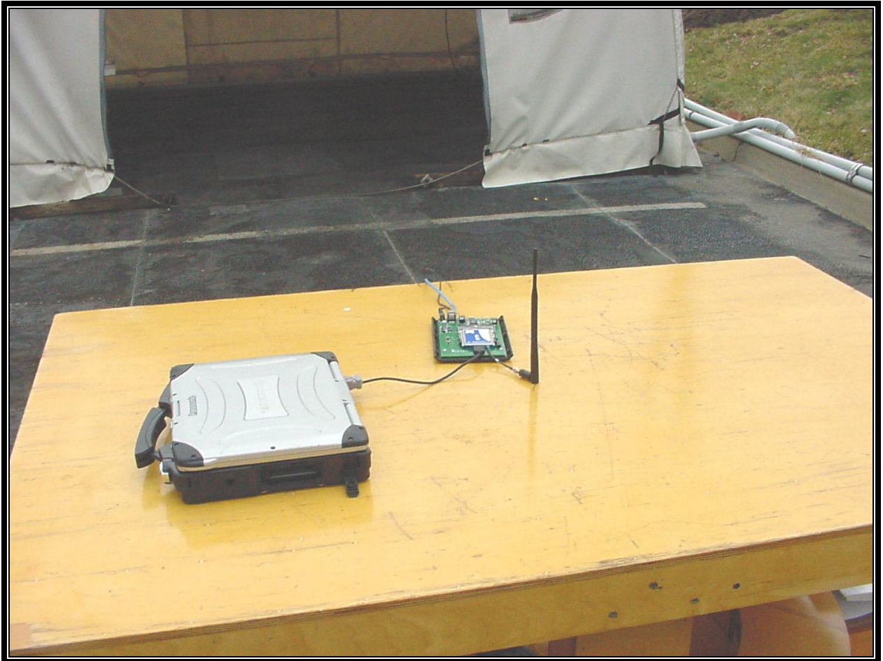
PHOTOGRAPH 3: RADIATED TEST CONFIGURATION ( \frac{1}{2} WAVE WHIP ANTENNA FRONT VIEW)
