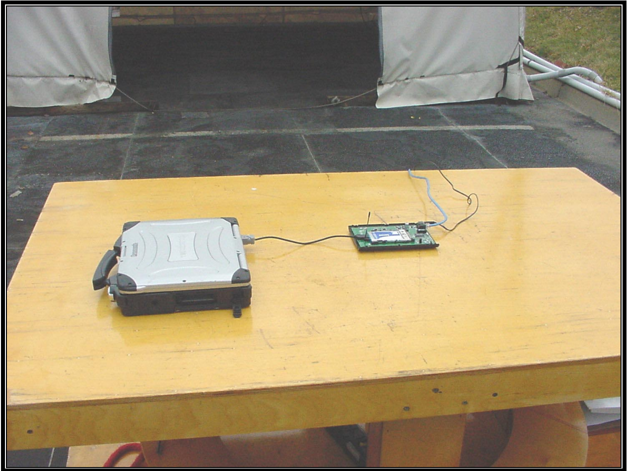
PHOTOGRAPH 1: RADIATED TEST CONFIGURATION ( \frac{1}{4} WAVE WHIP ANTENNA FRONT VIEW)
