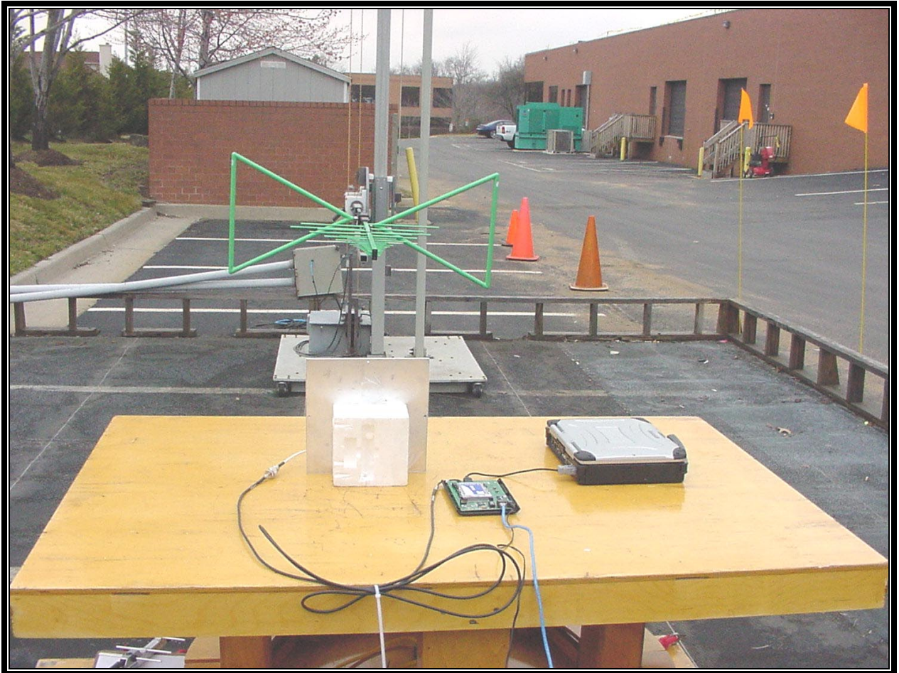
PHOTOGRAPH 6: RADIATED TEST CONFIGURATION (PATCH ANTENNA REAR VIEW)
