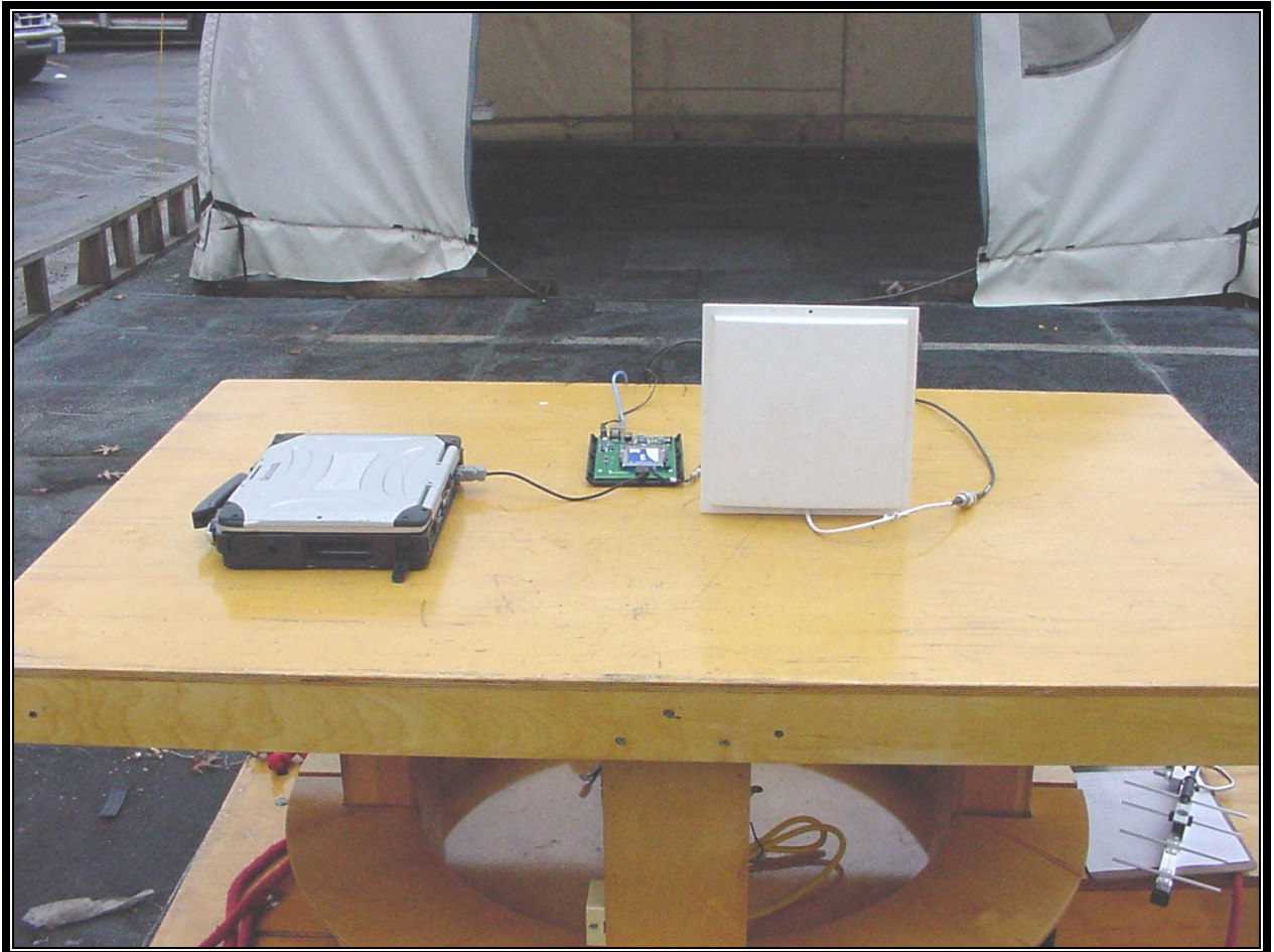
PHOTOGRAPH 5: RADIATED TEST CONFIGURATION (PATCH ANTENNA FRONT VIEW)
