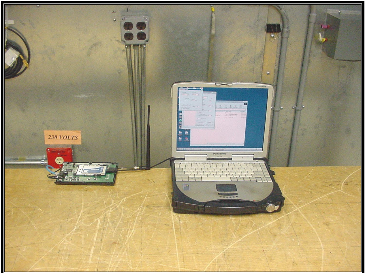
PHOTOGRAPH 11: CONDUCTED TEST CONFIGURATION ( \frac{1}{2} WAVE WHIP ANTENNA FRONT VIEW)
