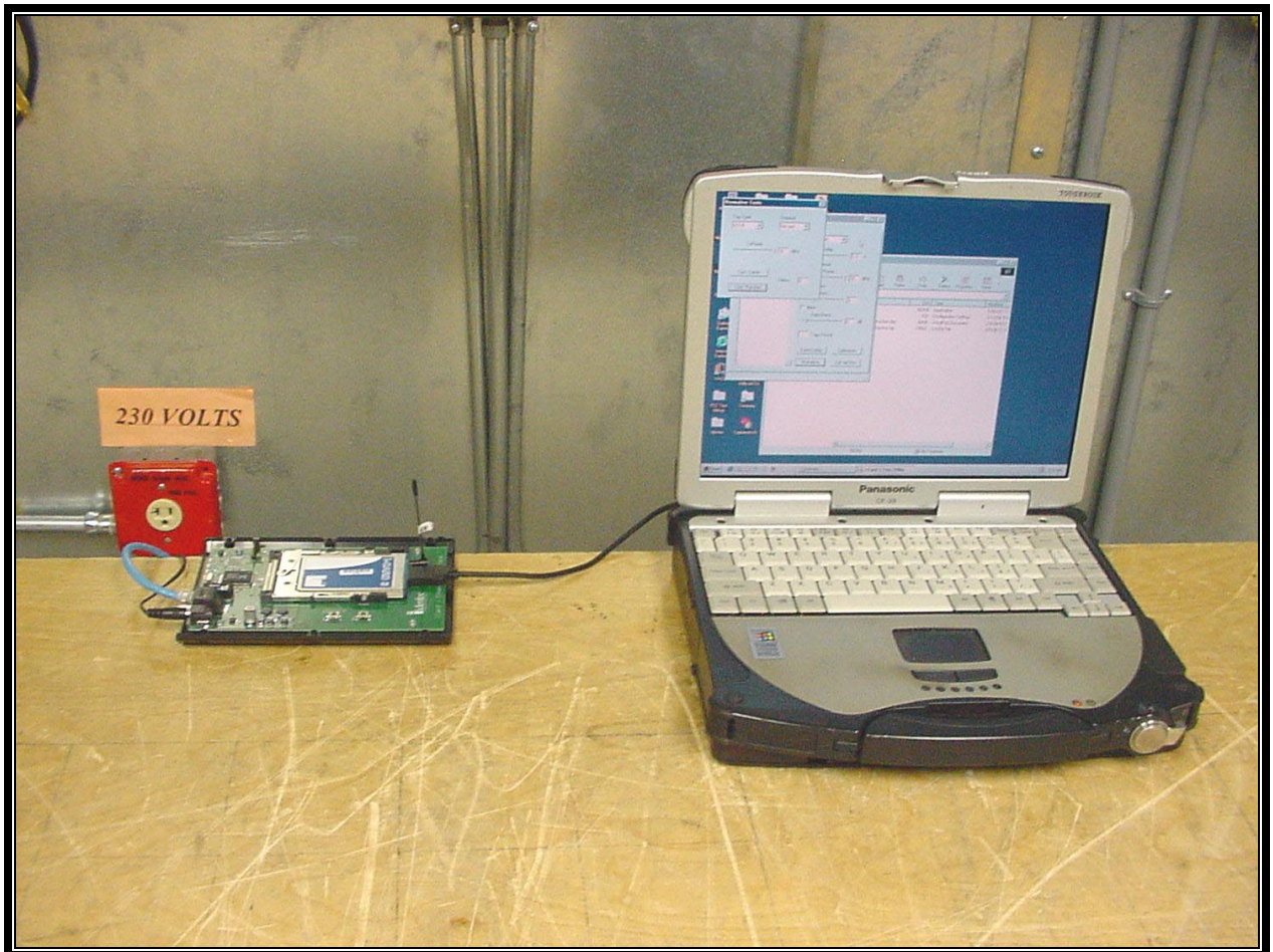
PHOTOGRAPH 9: CONDUCTED TEST CONFIGURATION (1/4 WAVE WHIP ANTENNA FRONT VIEW)
