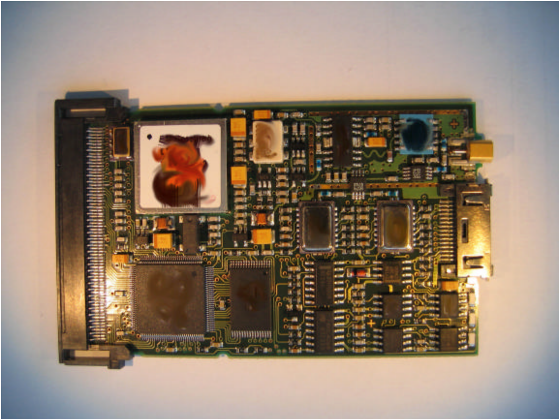
PCMCIA Card Without Shields - Top View
