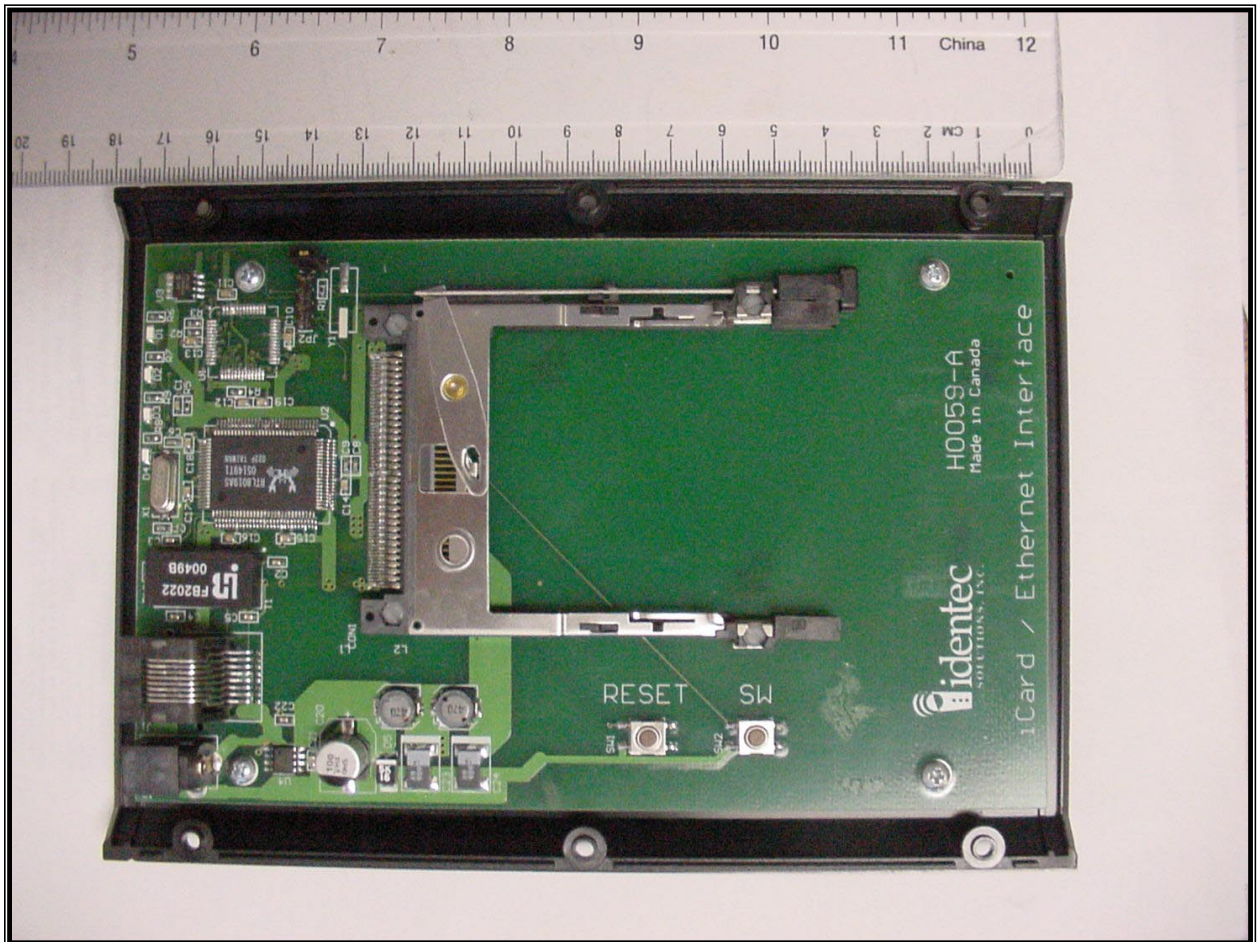
PHOTOGRAPH 23: PCB MOUNTED WITHOUT PCMCIA CARD
