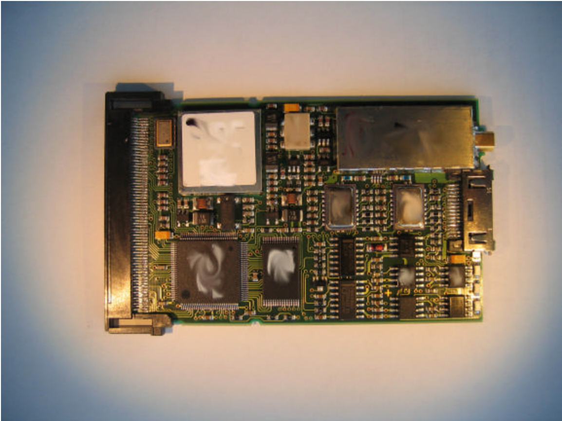
PCMCIA Card with Shields - Top View
