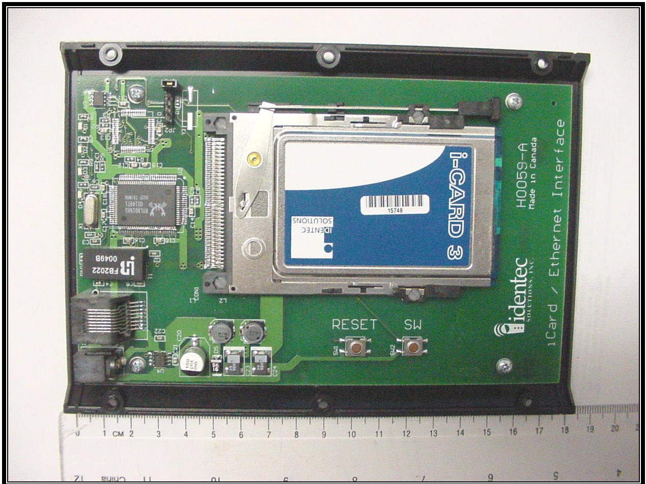
PHOTOGRAPH 24: PCB MOUNTED WITH PCMCIA CARD
