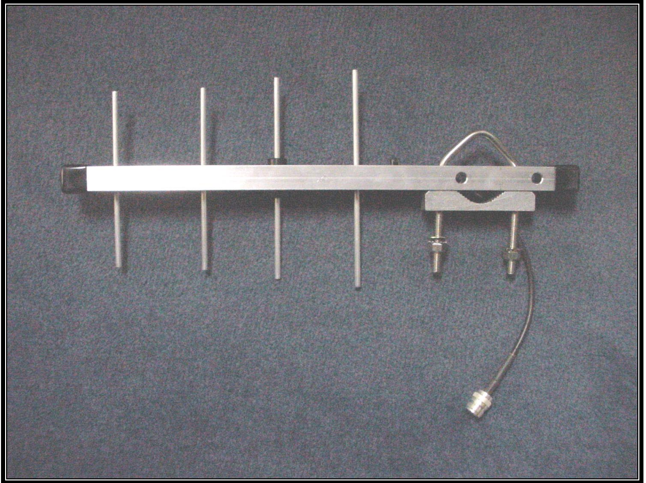
PHOTOGRAPH 19: YAGI ANTENNA TOP VIEW
