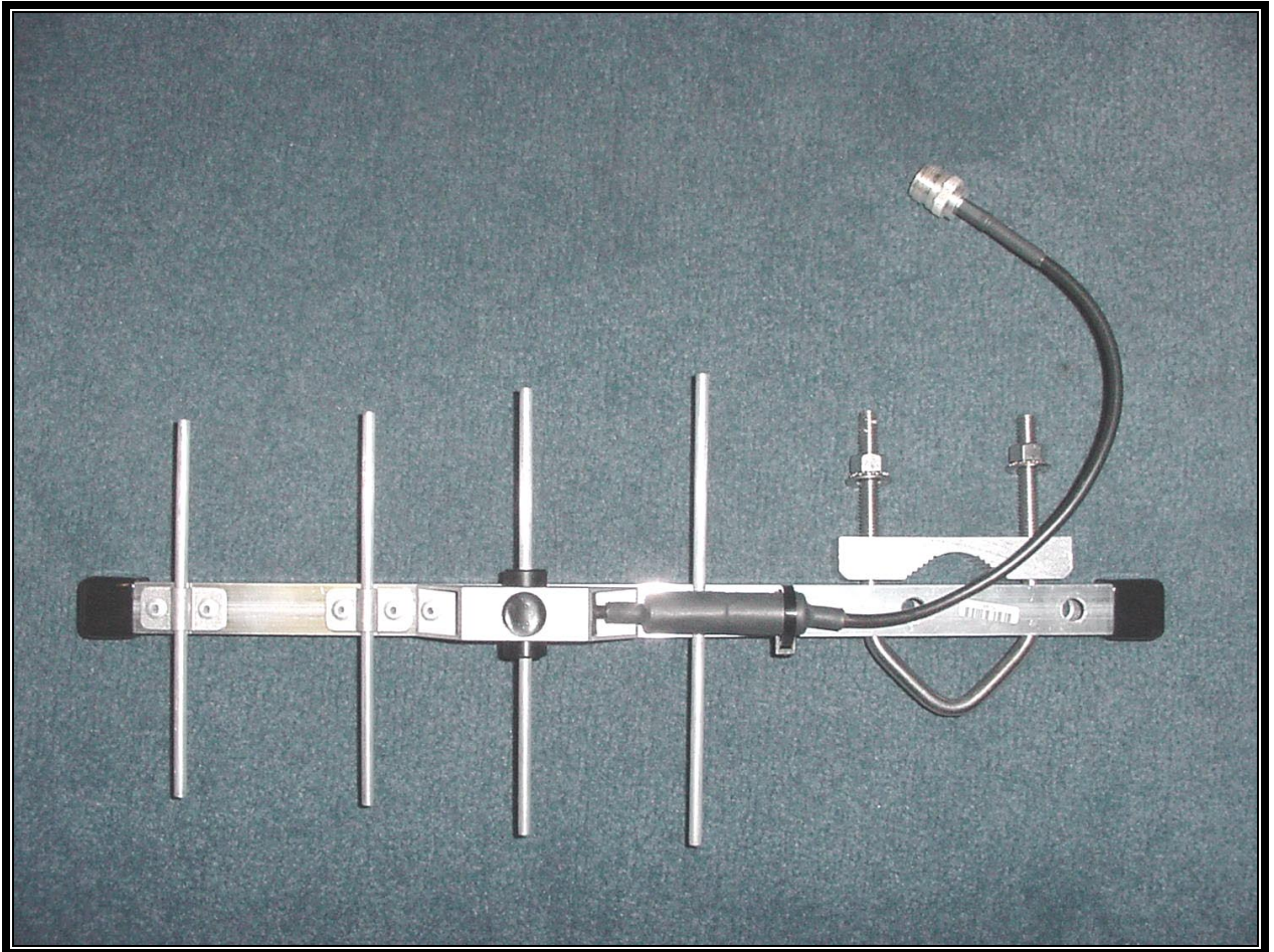
PHOTOGRAPH 20: YAGI ANTENNA BOTTOM VIEW
