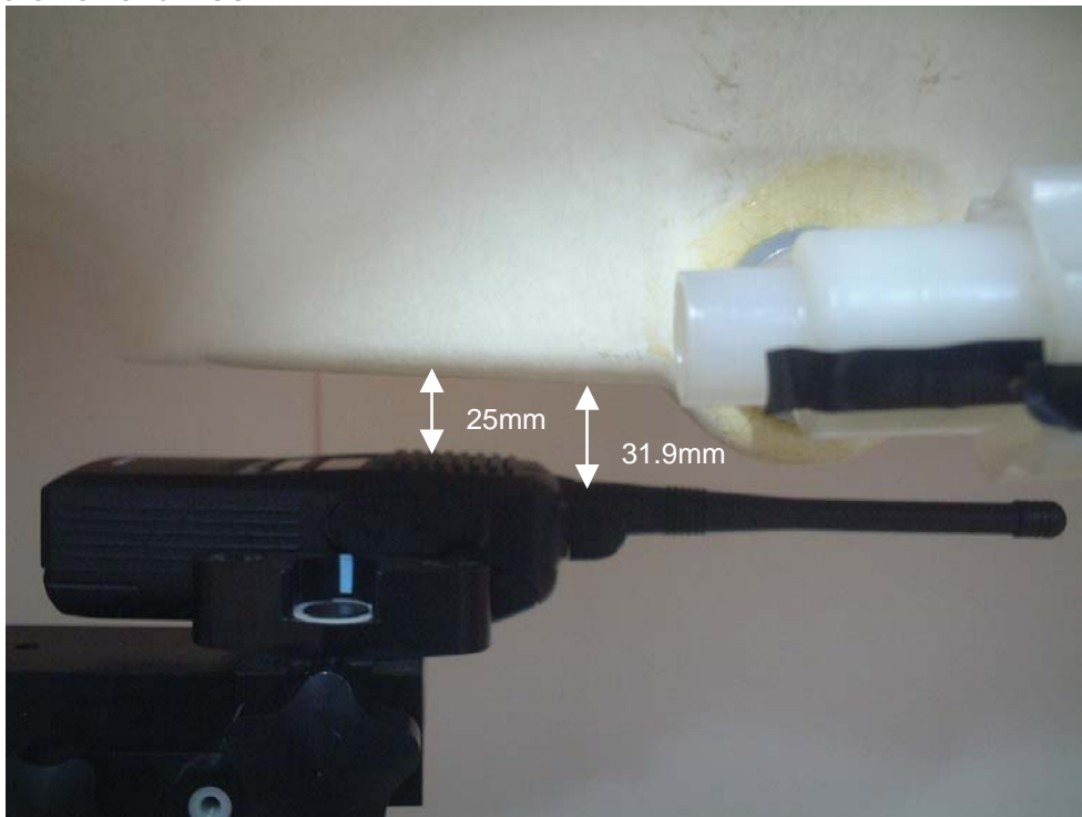
* Body worn of O25PJ-100NW
